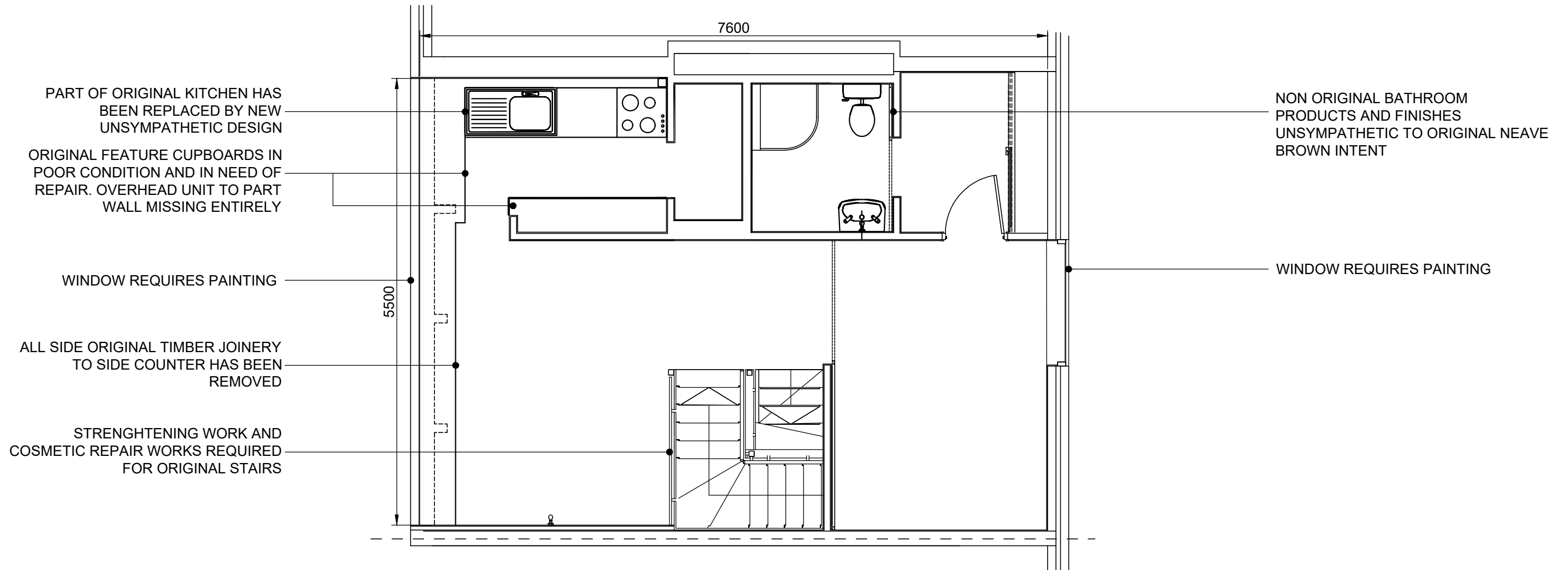
01 SCALE 1:50 EXISTING FIRST FLOOR PLAN
