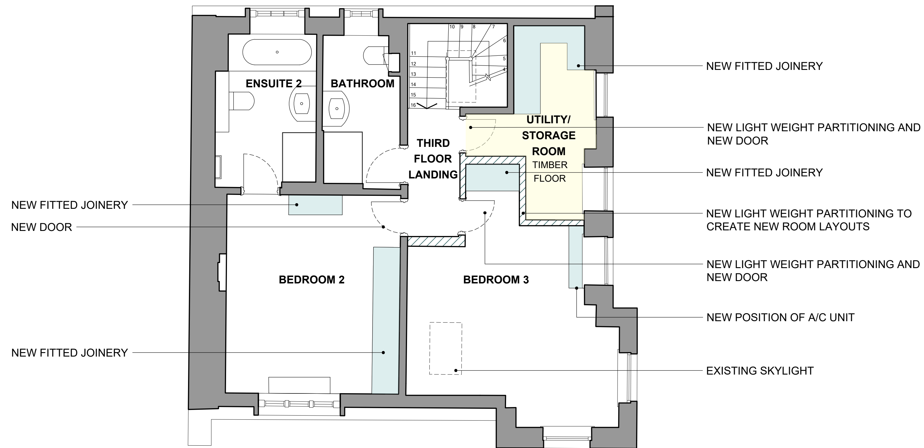
01 THIRD FLOOR PLAN 1:50 @ A1
