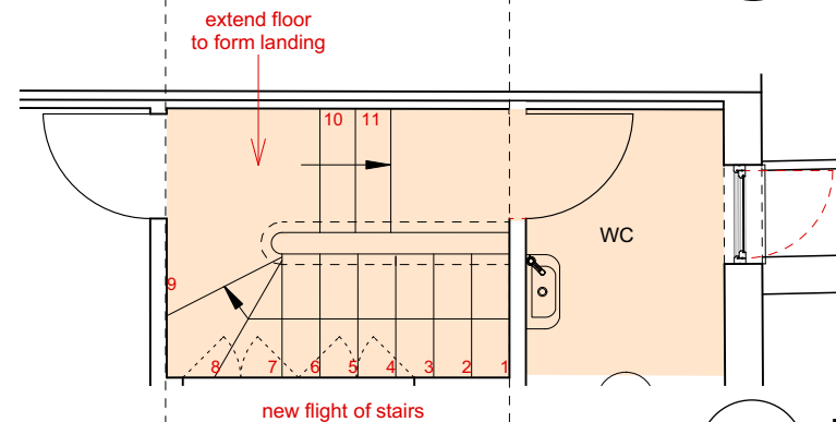
04 Proposed loft plan 23 1:50@A3; 1:25@A1
