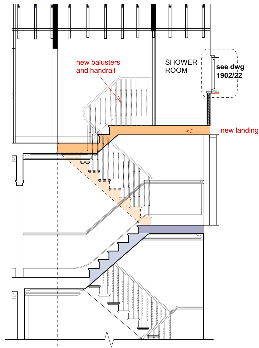
06 Proposed section A-A 23 1:50@A3; 1:25@A1
