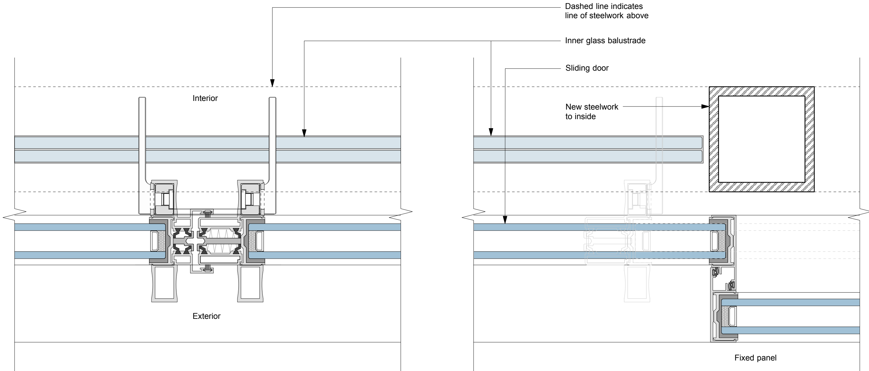
Detail A_ Door Junction
