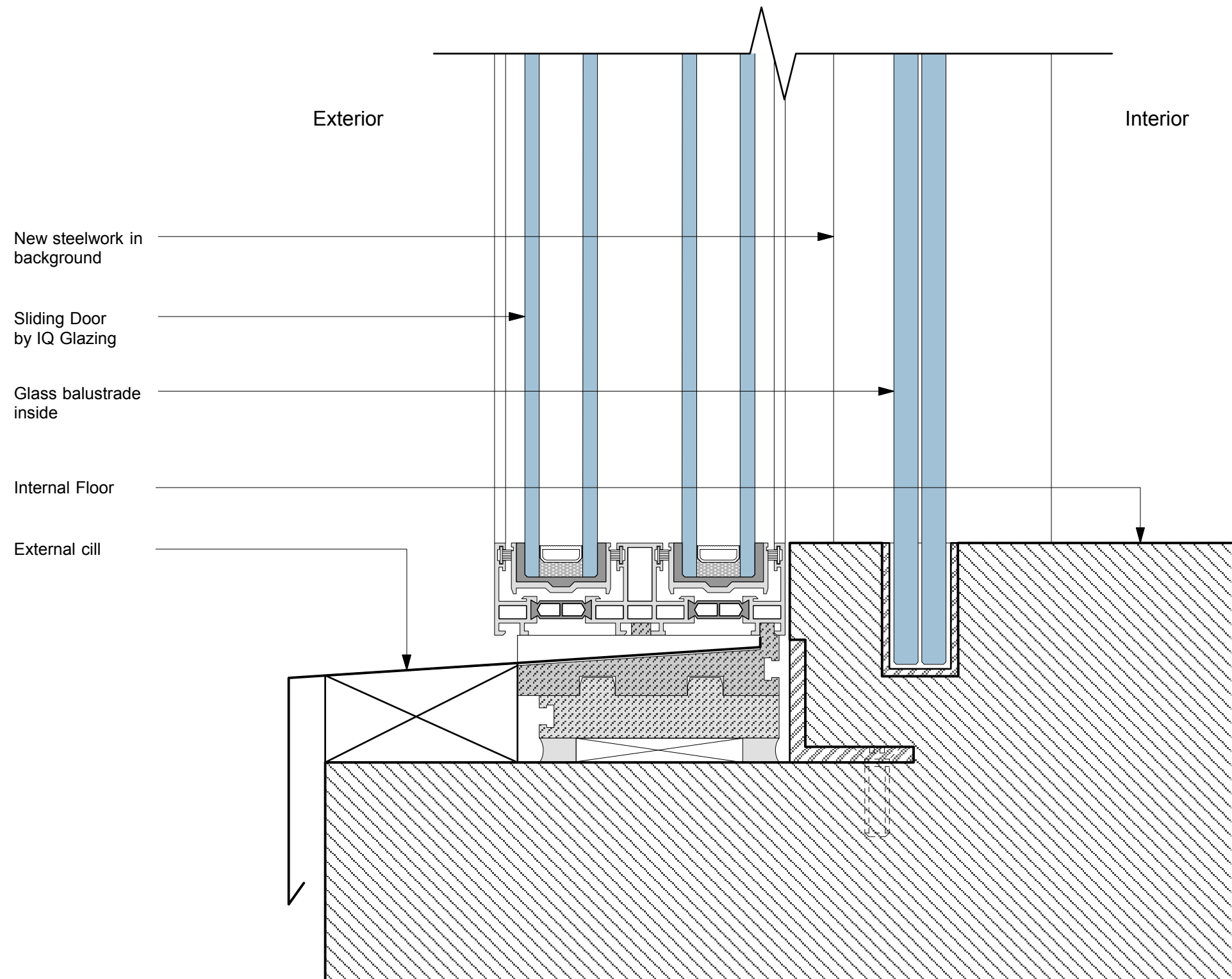
Detail C _ Threshold
