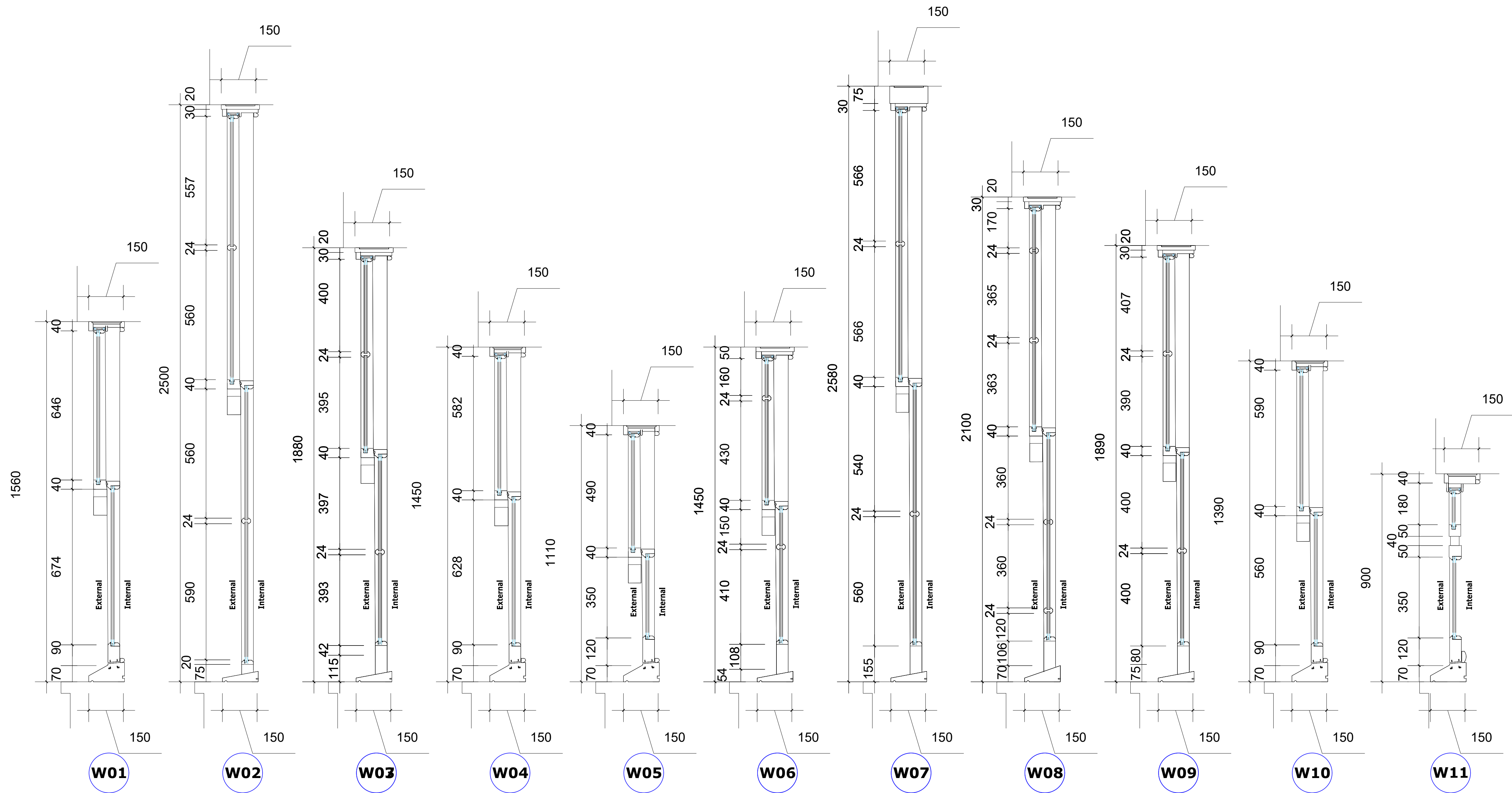
1 Existing Window Section Scale 1:10 @ A1
