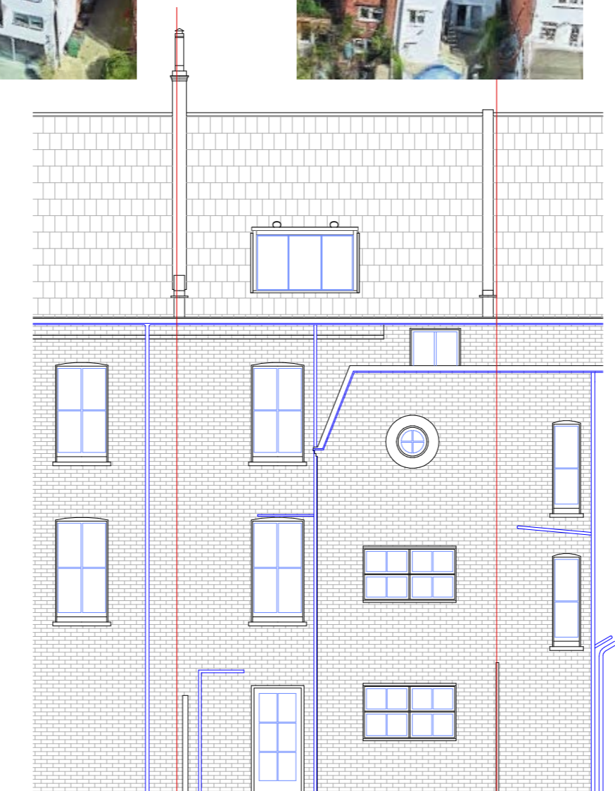
REAR ELEVATION
