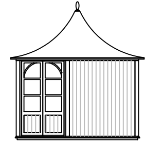
South West Elevation
