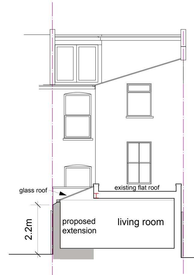
SECTION CC
