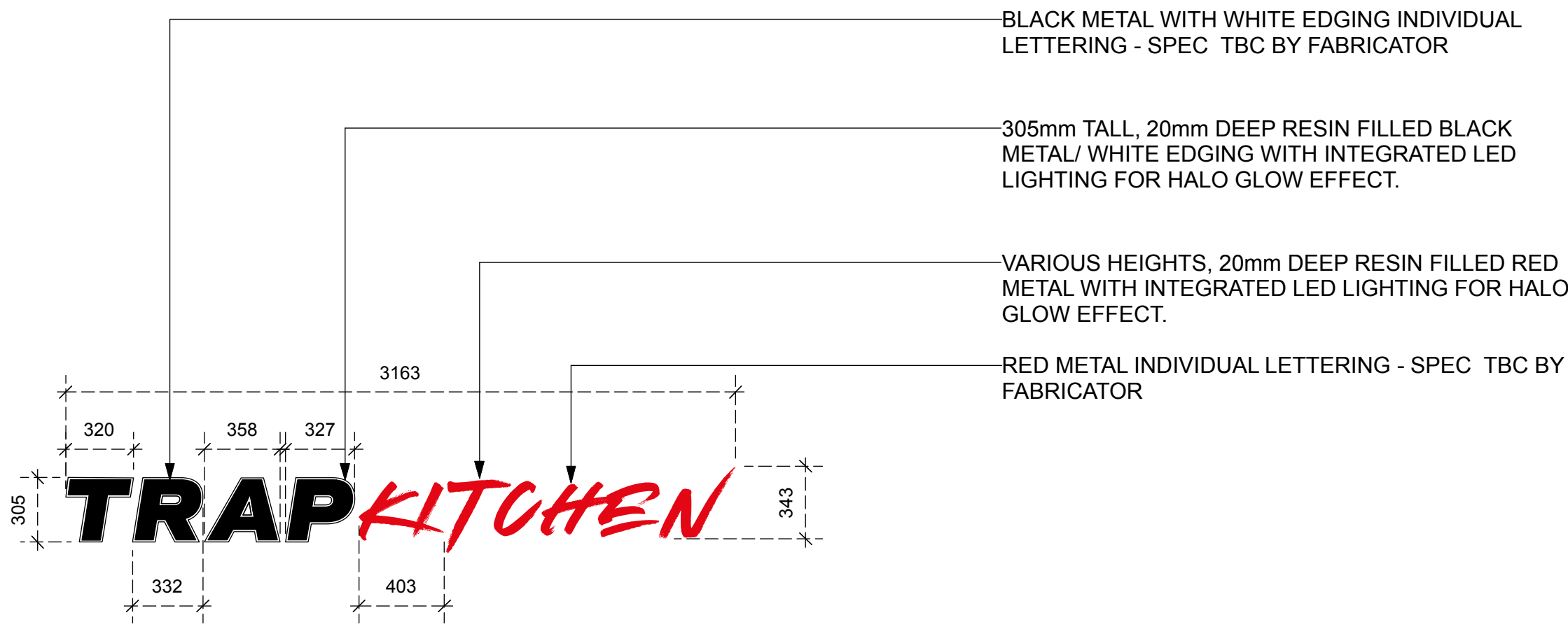
1 EXTERNAL SIGNAGE - TRAP KITCHEN Scale: 1:50 @ A3
