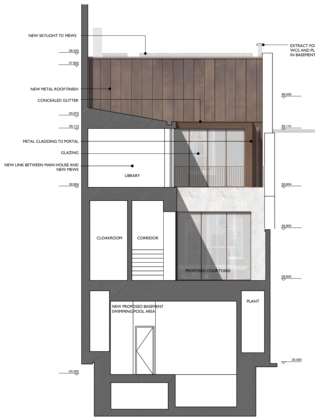
SECTION EE
