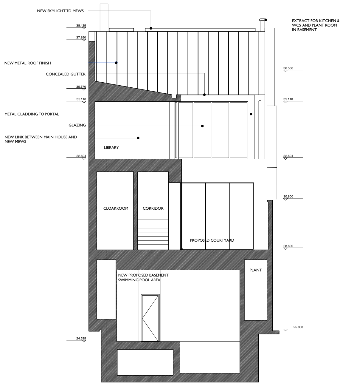
SECTION EE
