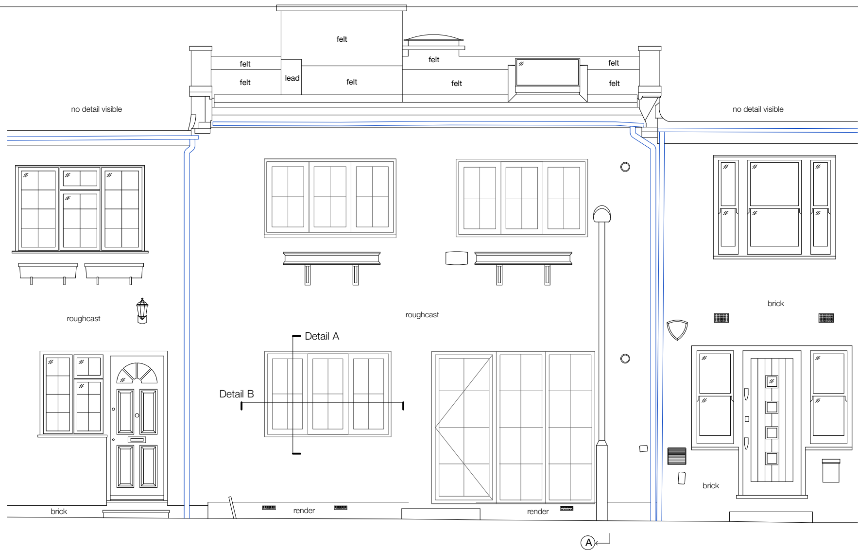
FRONT ELEVATION (South East) Reproduced as key reference, refer to Drawing P200
