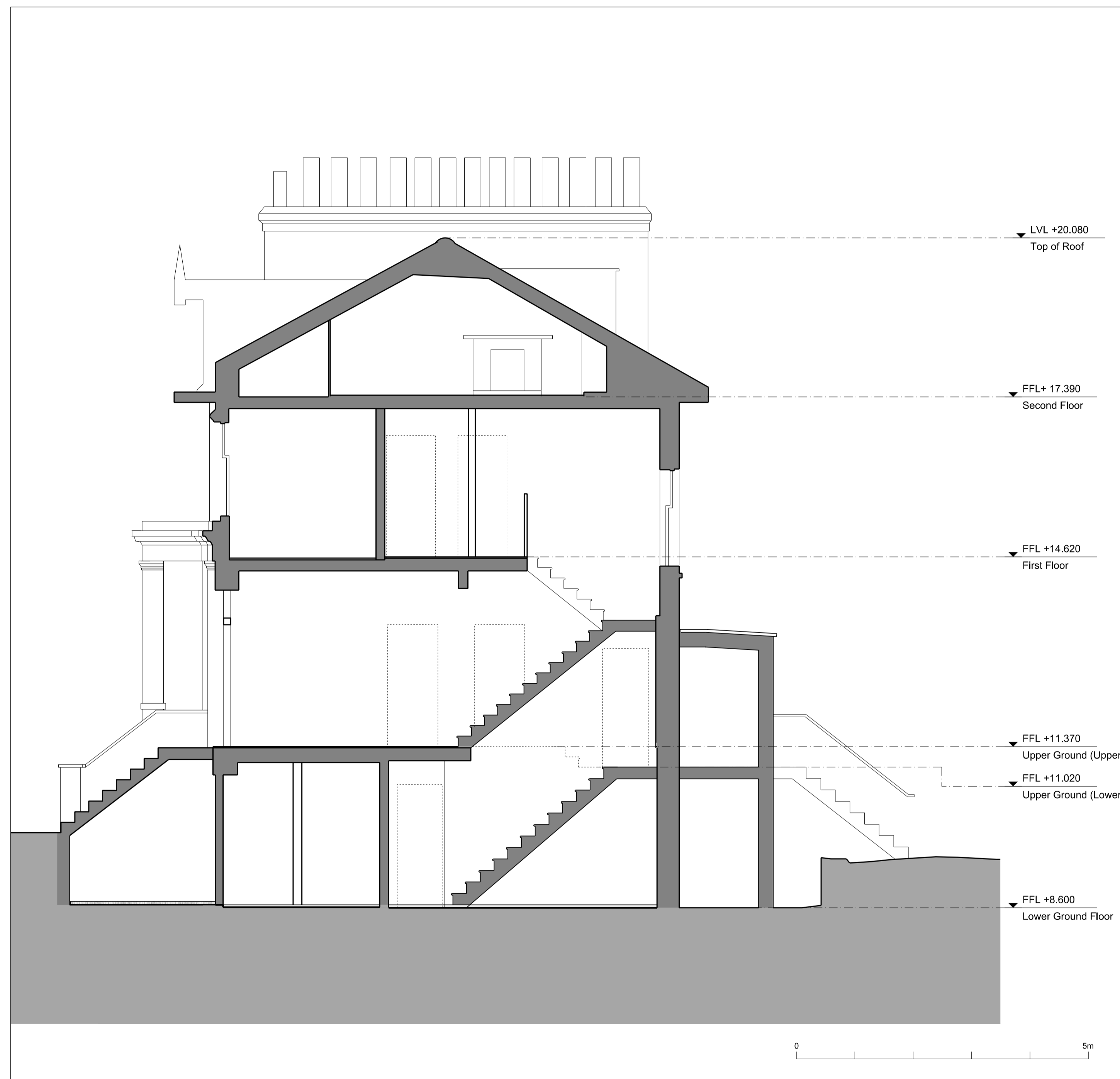
01 Existing Section C 1:50 @ A1
