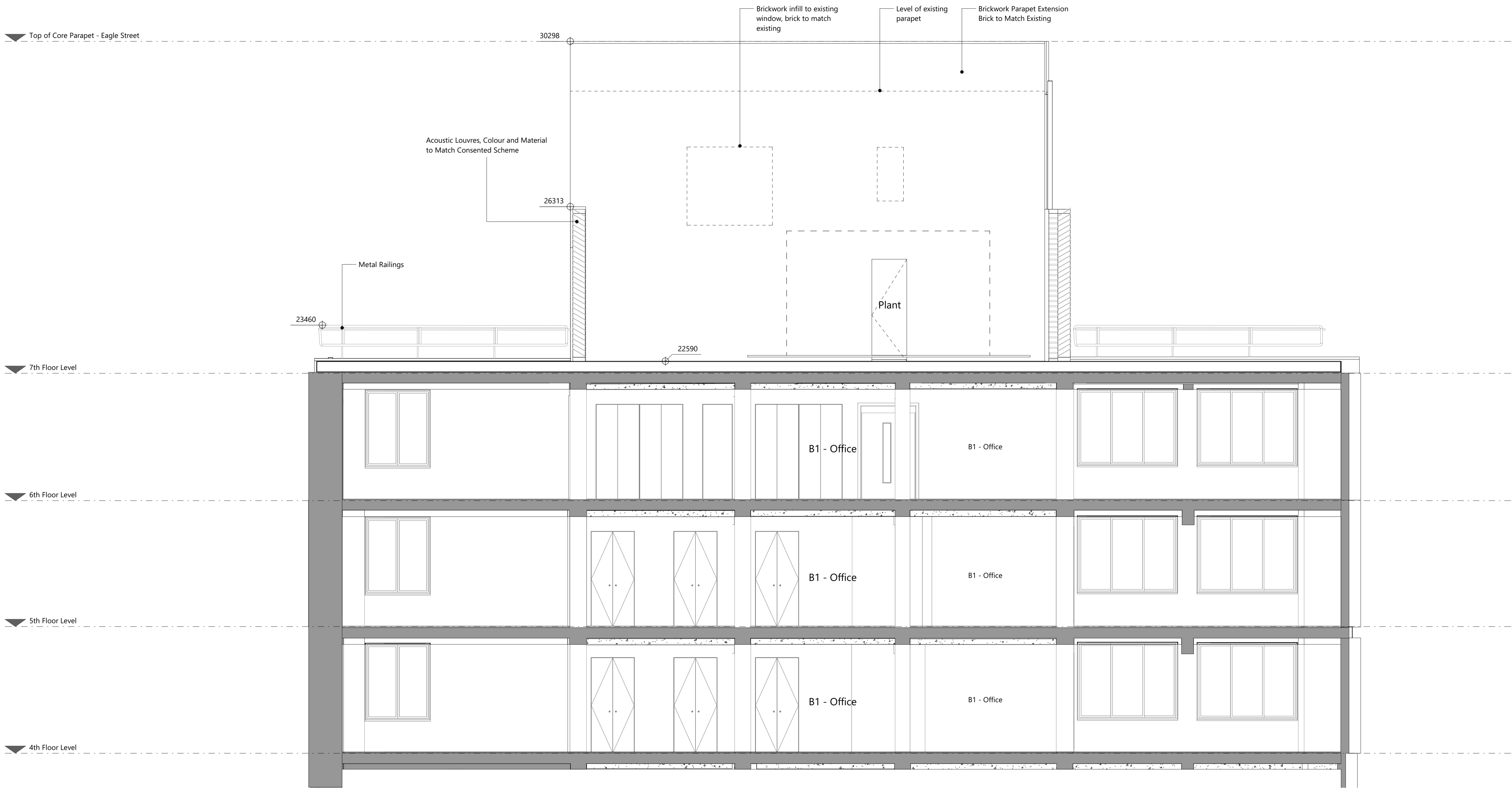
1 Plant Enclosures Section DD
