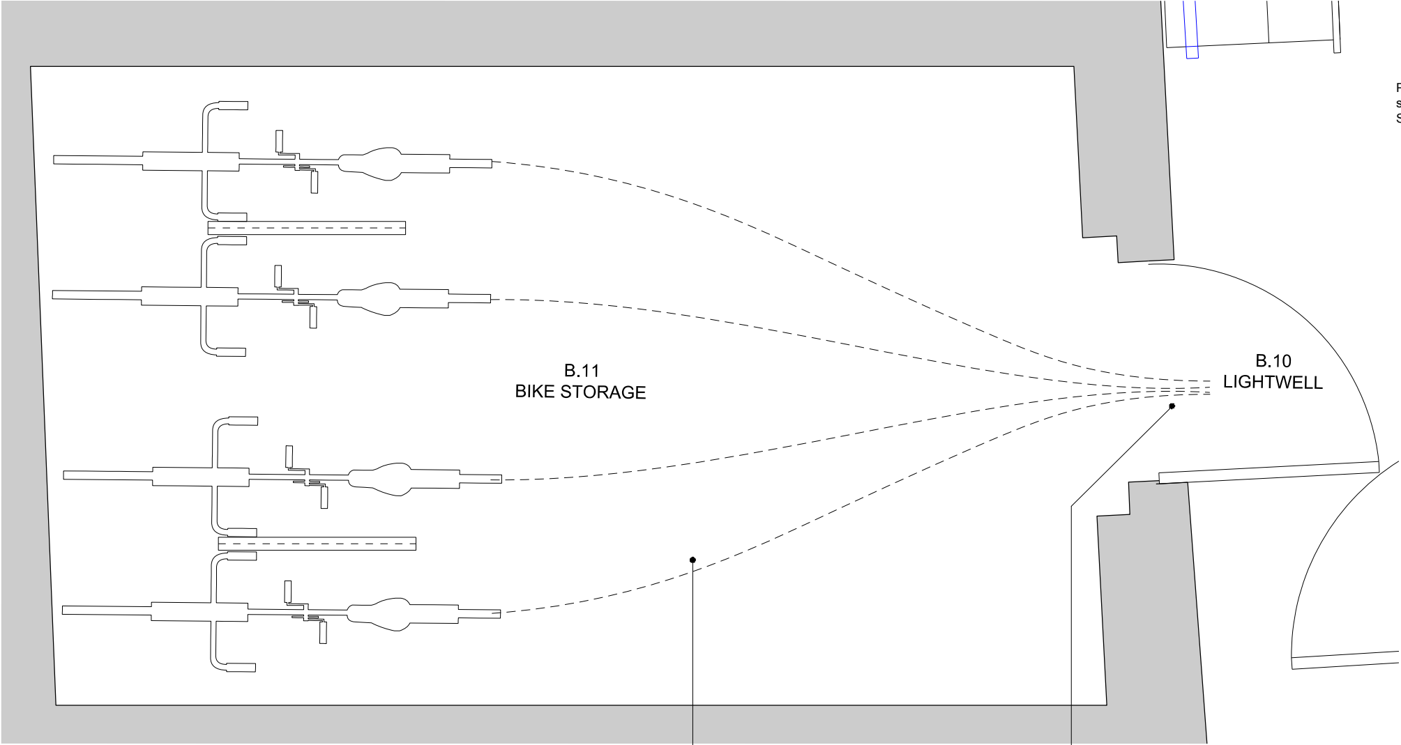
Plan: vault B.11 - bike store for 4no. bikes with Sheffield Bike Stands Scale 1:20
