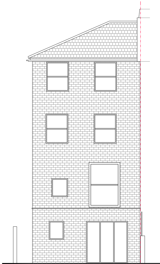
EXISTING REAR ELEVATION (Remains as existing)
