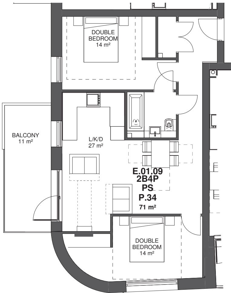
Type P.34 - 2B4P Private
