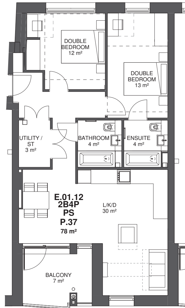
Type P.37 - 2B4P Private
