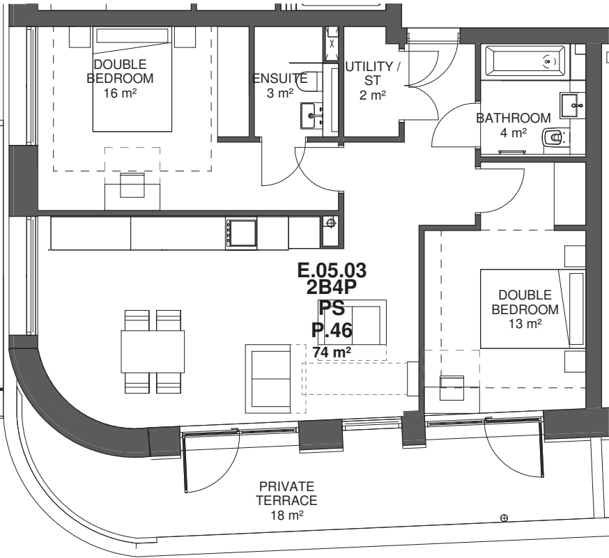
Type P.46 - 2B4P Private
