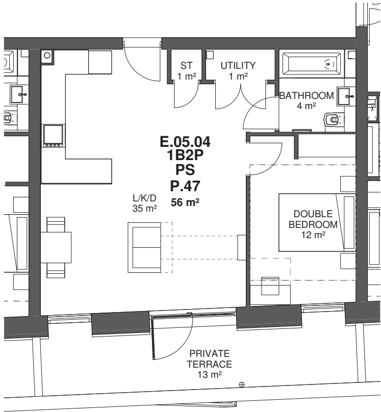
Type P.47 - 1B2P Private
