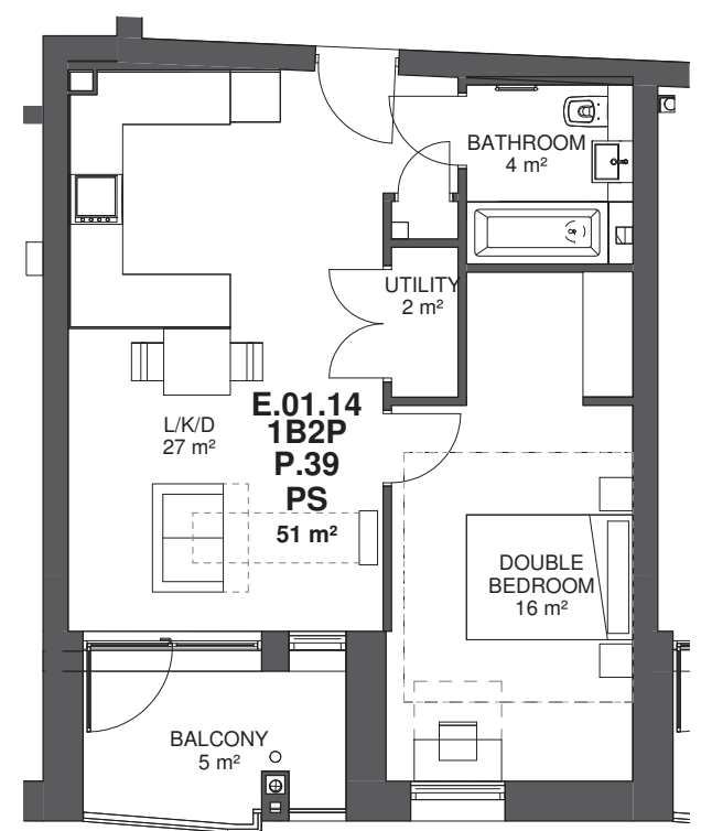
Type P.39 - 1B2P Private
