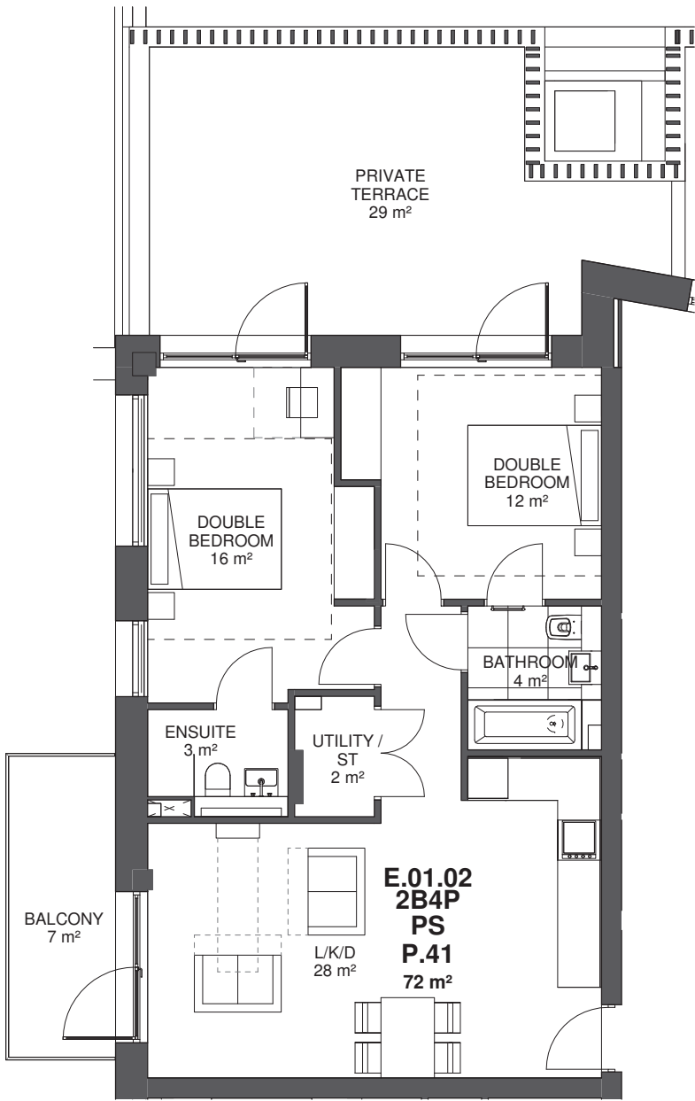
Type P.41 - 2B4P Private
