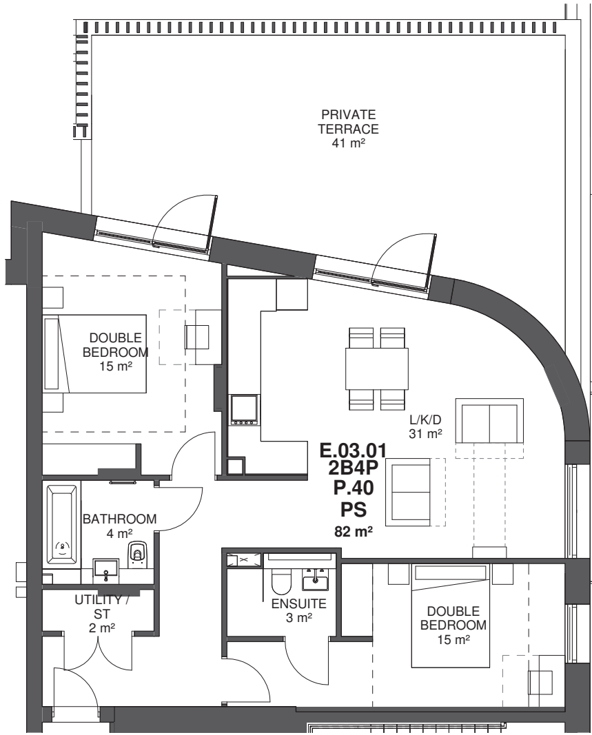
Type P.40 - 2B4P Private
