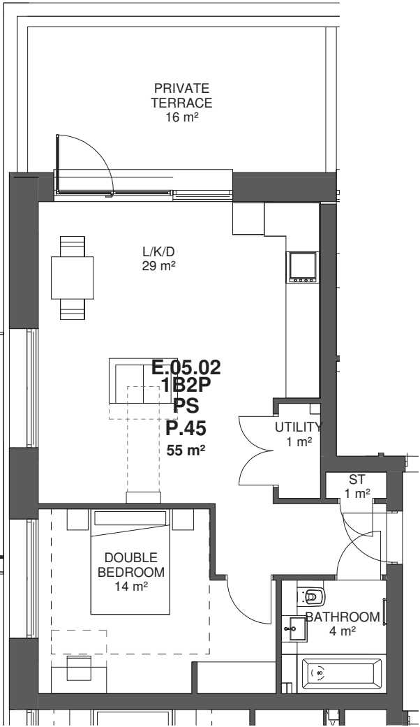
Type P.45 - 1B2P Private
