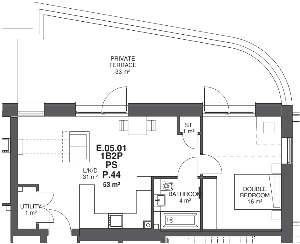
Type P.44 - 1B2P Private
