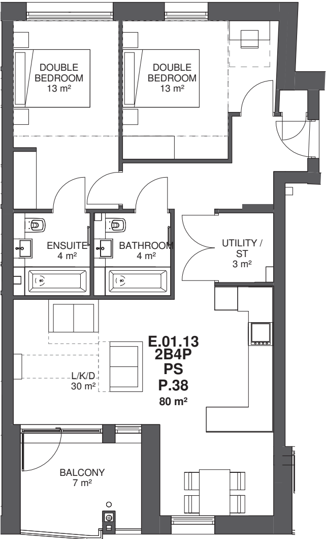
Type P.38 - 2B4P Private
