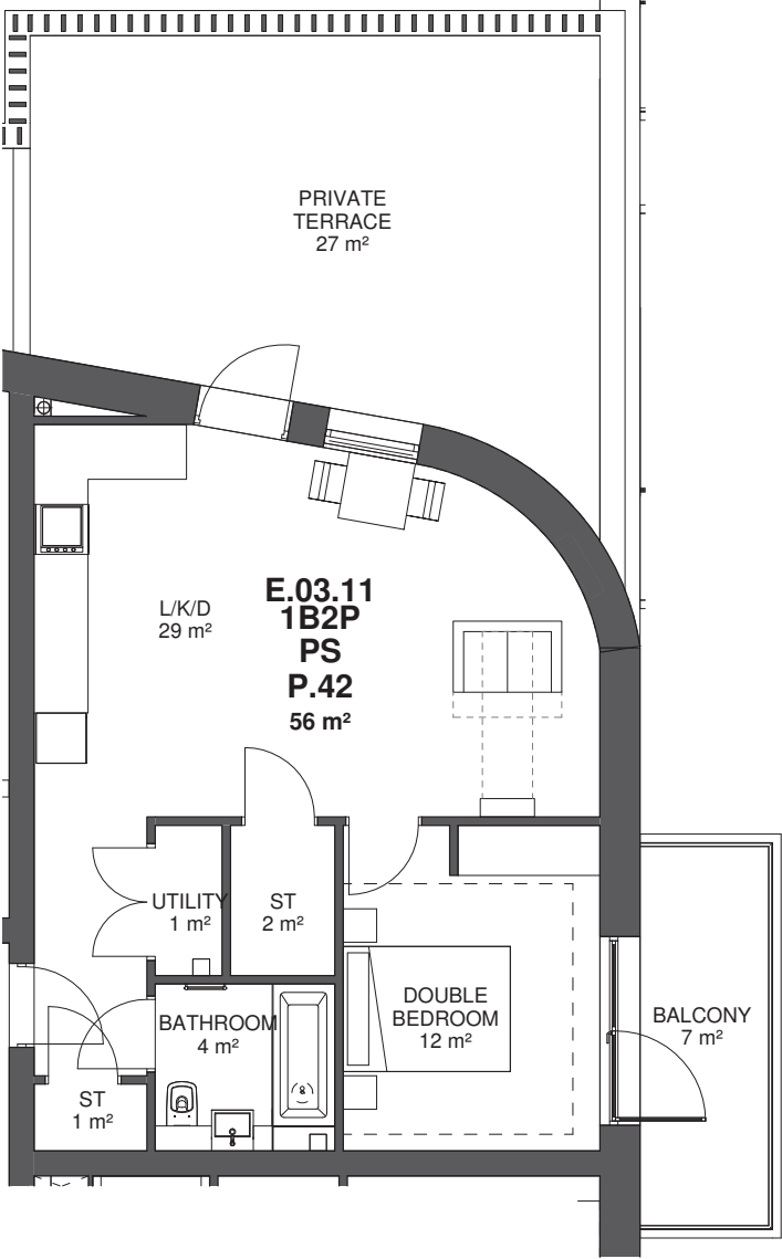
Type P.42 - 1B2P Private
