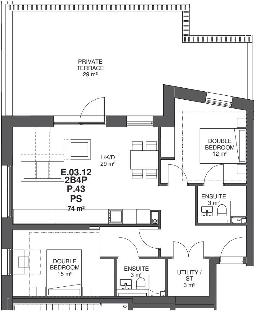
Type P.43 - 2B4P Private
