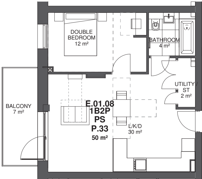
Type P.33 - 1B2P Private
