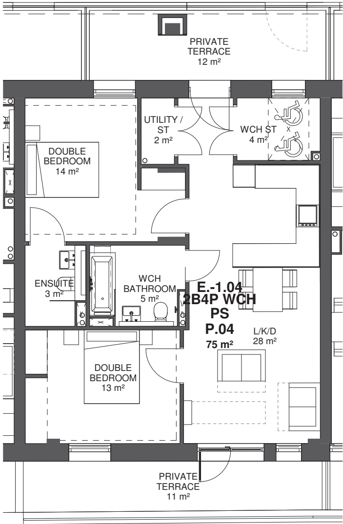
Type P.04 - 2B4P WCH Private
