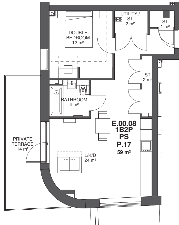
Type P.17 - 1B2P Private
