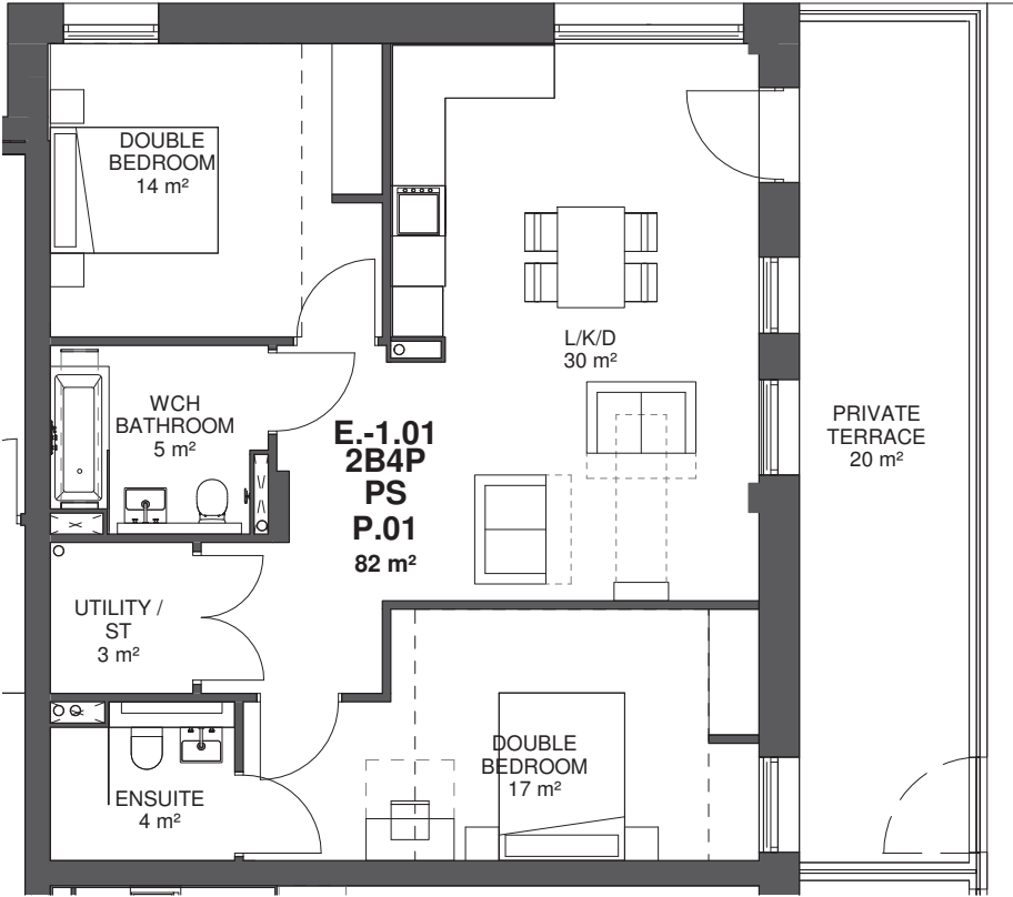
Type P.01 - 2B4P Private
