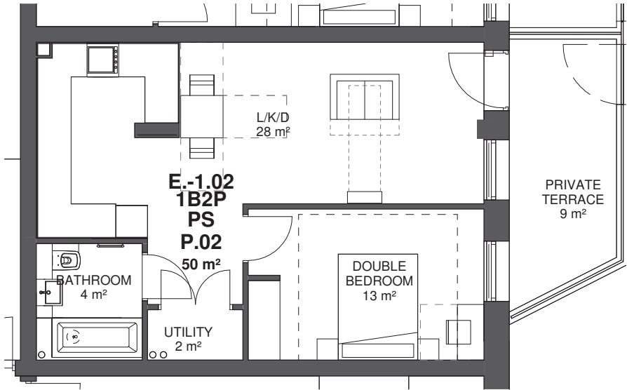
Type P.02 - 1B2P Private
