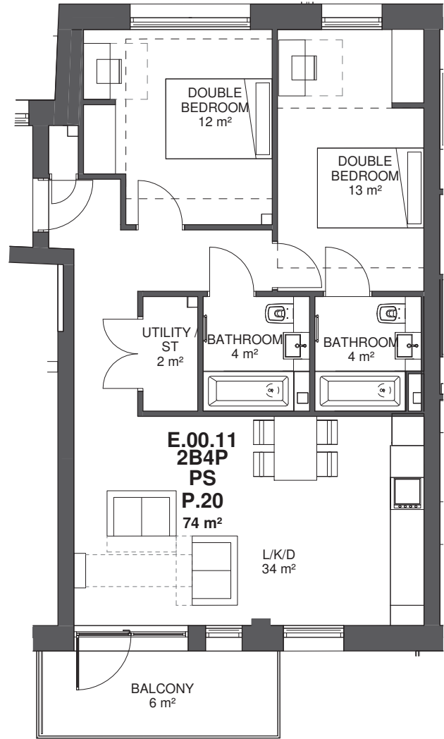
Type P.20 - 2B4P Private
