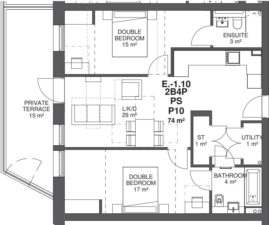
Type P.10 - 2B4P Private
