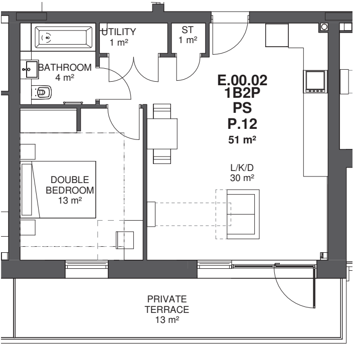
Type P.12 - 1B2P Private
