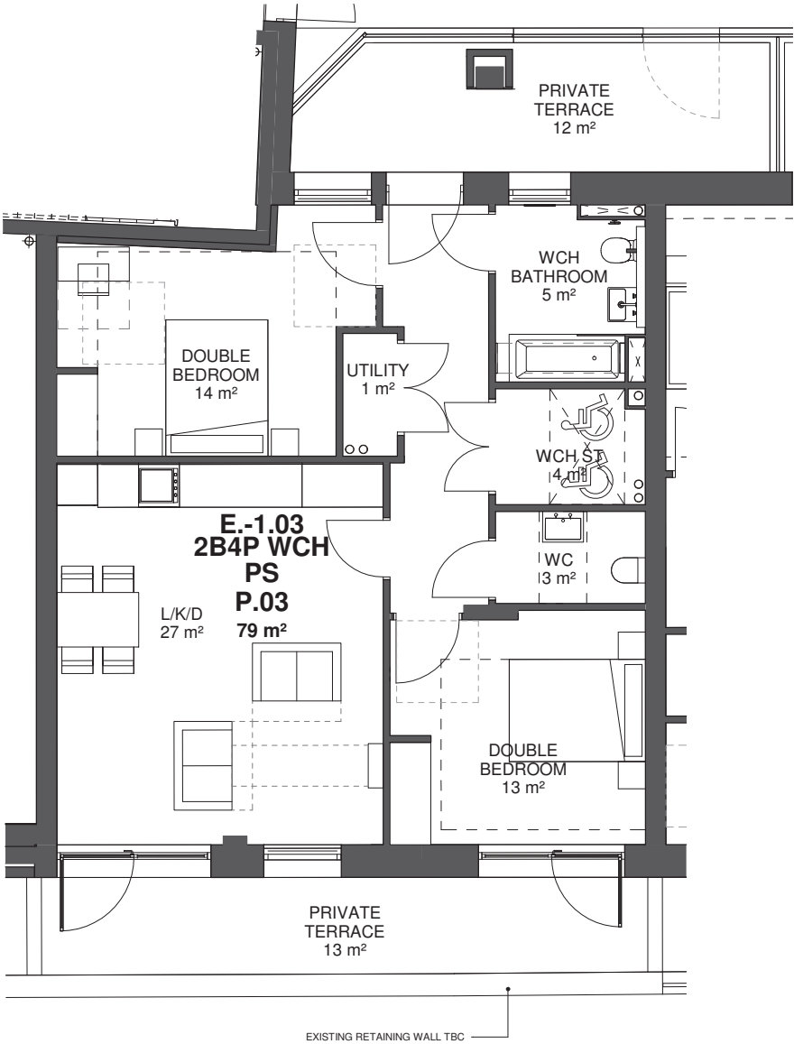
Type P.03 - 2B4P WCH Private
