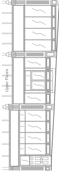
EXISTING FRONT ELEVATION Scale 1:50
