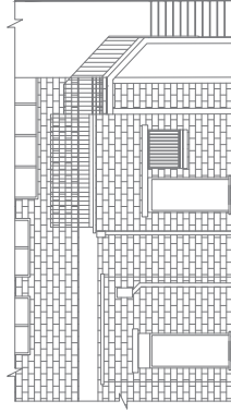
PROPOSED REAR ELEVATION Scale 1:50
