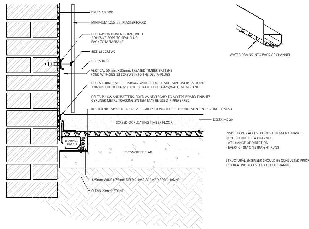
Indicative Delta lining membrane and drain detail (Main Basement Area)
