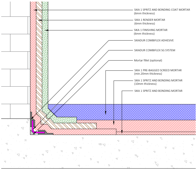
Indicative Sika Render tanking system detail (Pavement Vault Area)
