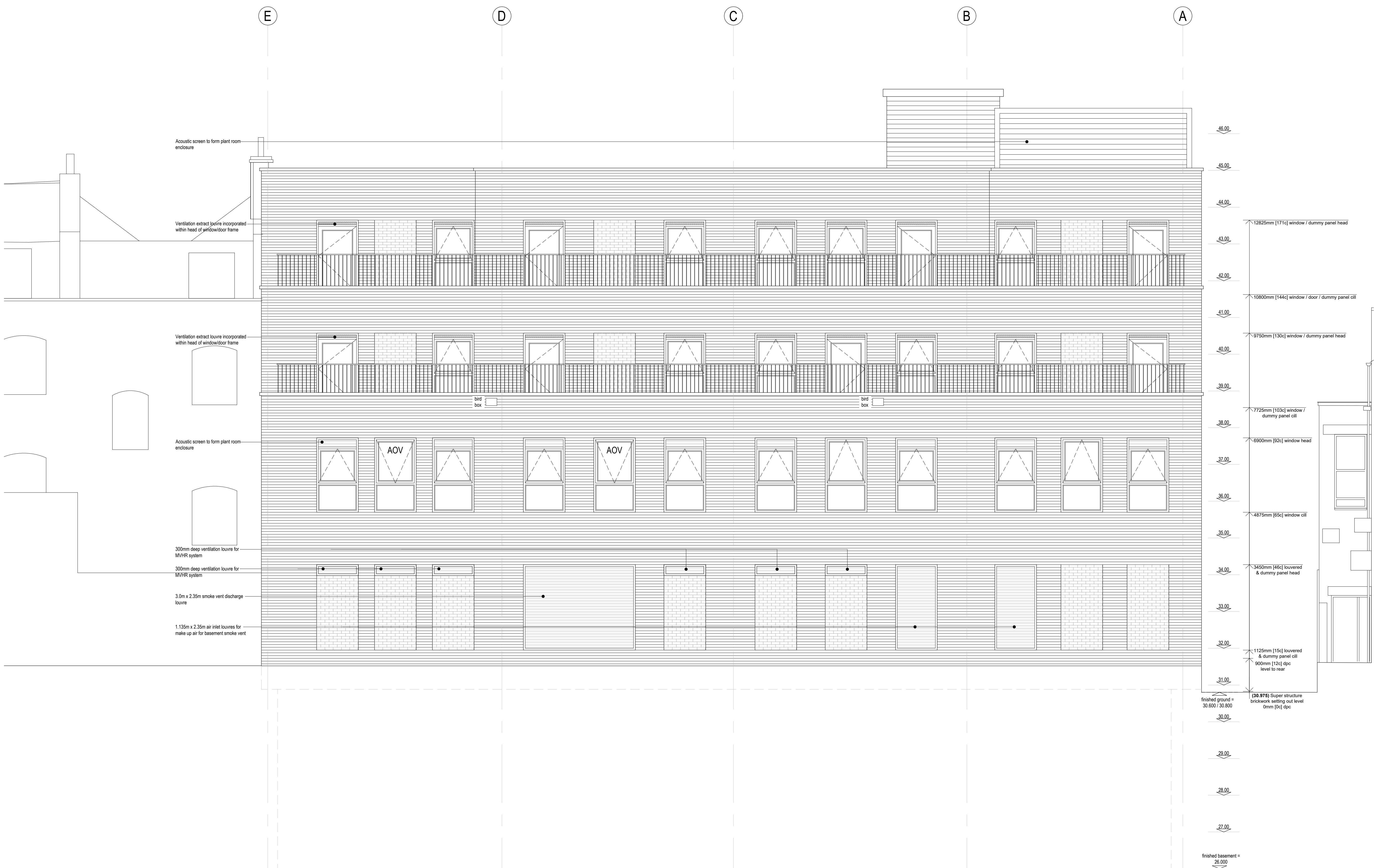
proposed rear (east) elevation
