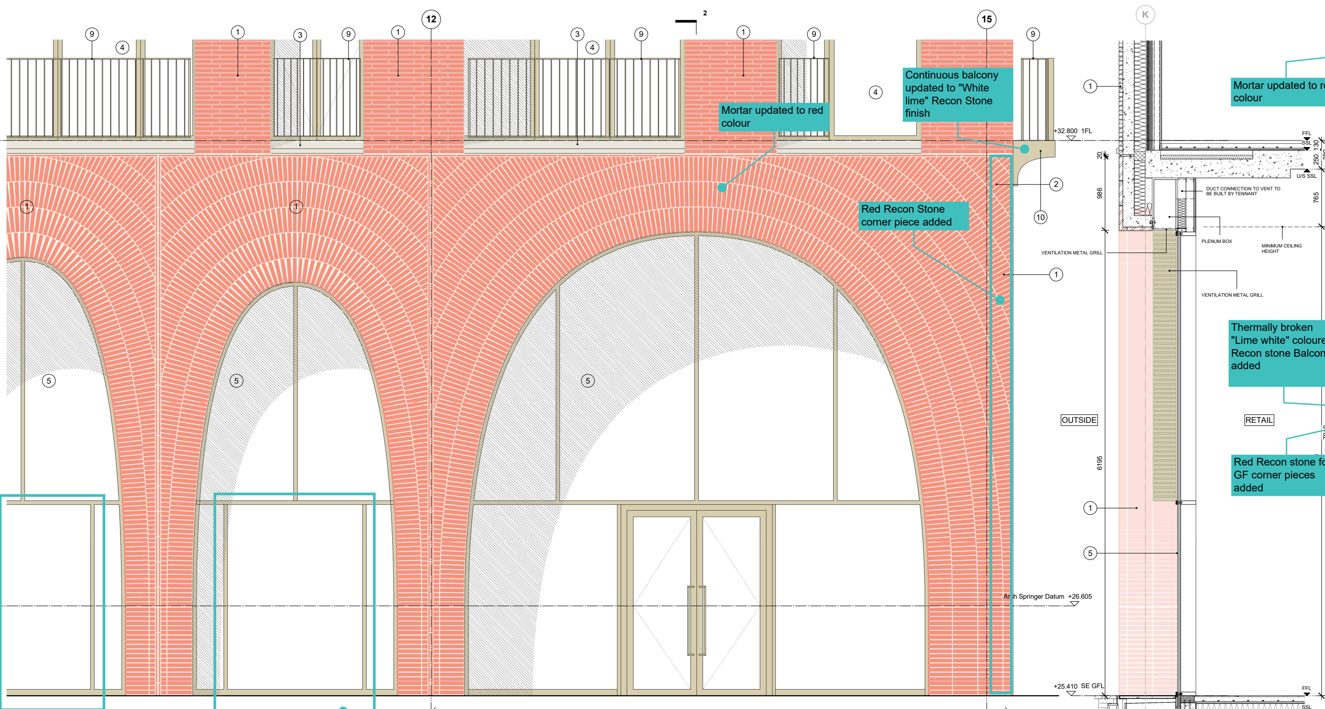
1 ELEVATION DETAIL SOUTH FACADE, TYPICAL RETAIL
