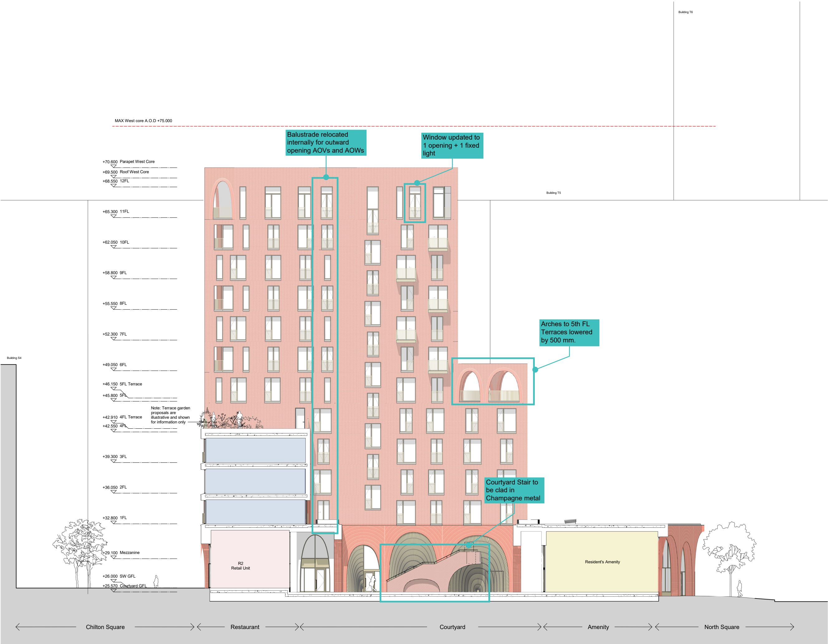
1 Internal West Core Elevation
