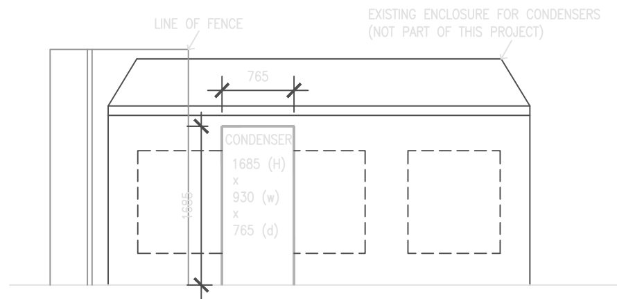
ELEVATION 1 – CONDENSER SIZE
