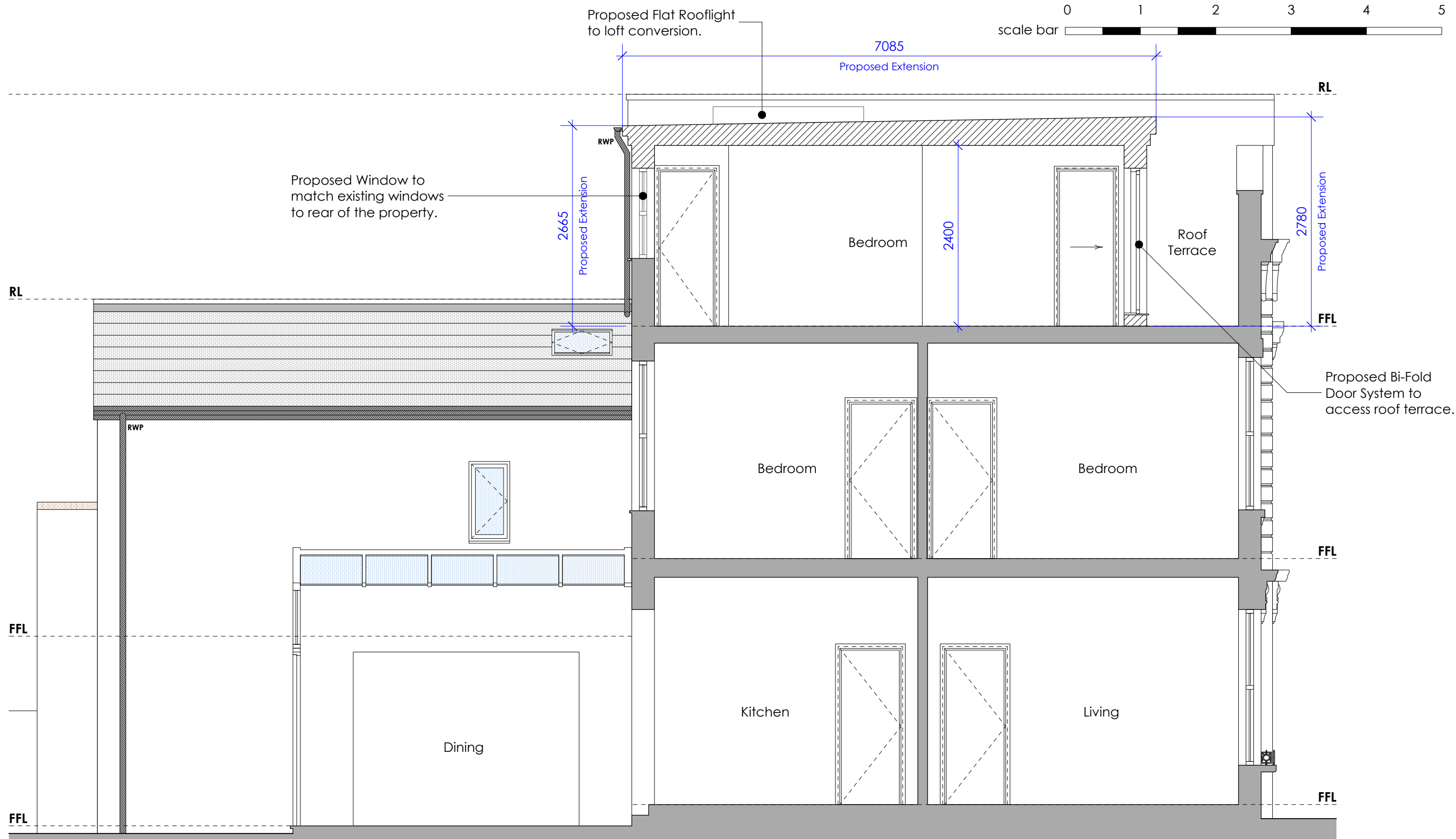
1 Proposed Section & Side Elevation scale: 1:50 @ A3
