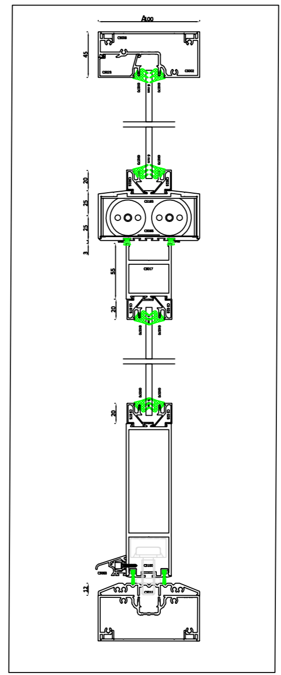
<<<<FULL HEIGHT CUT THROUGH - CUT A>>>>
