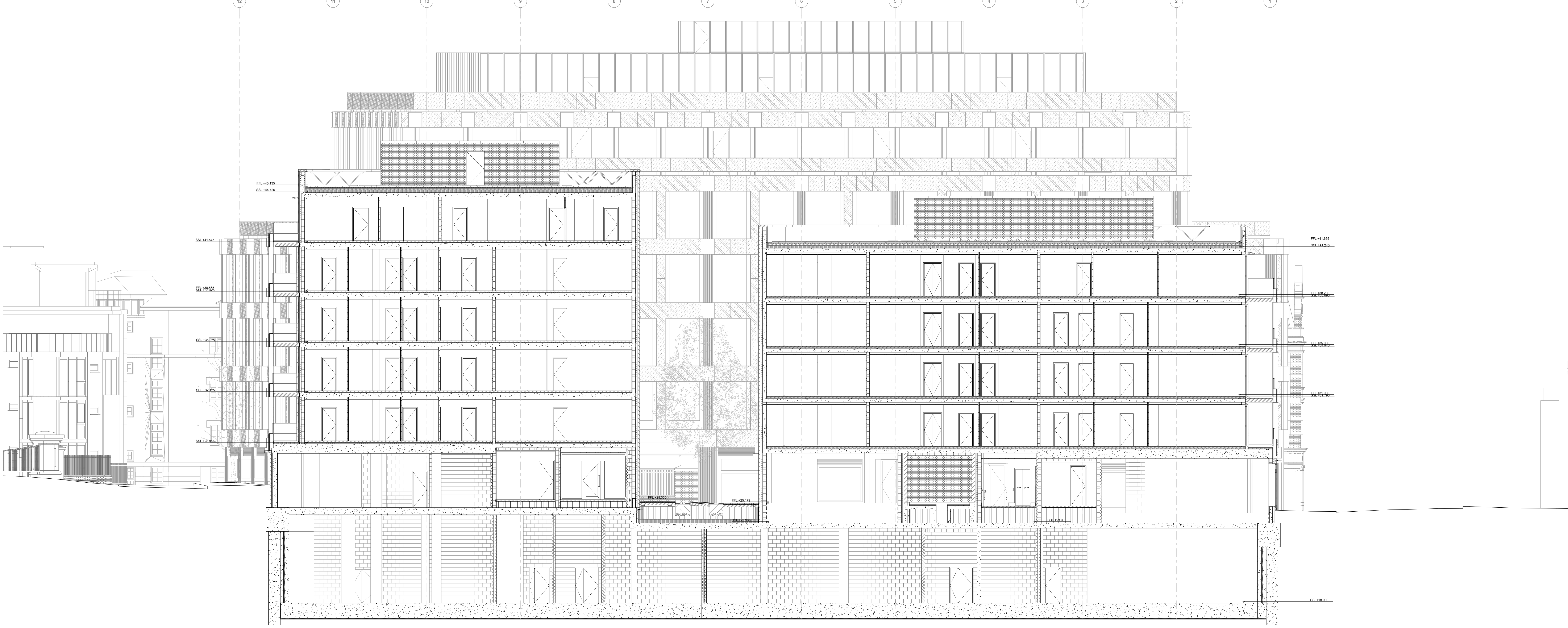
Section AA1
