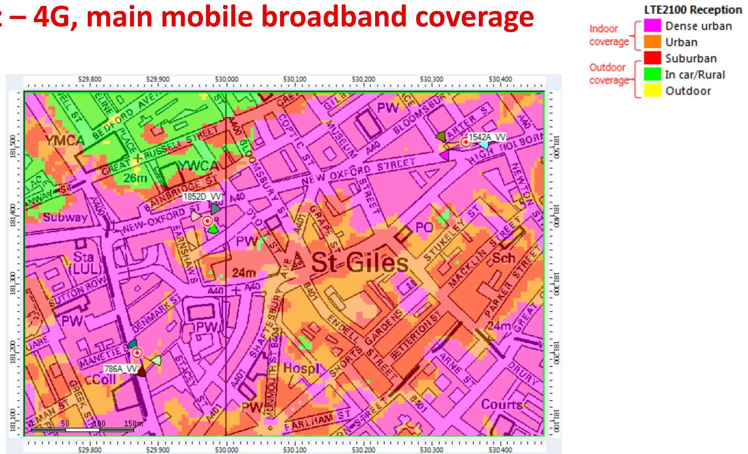
Fig. 4: Former LTE2100MHz, main mobile broadband coverage
