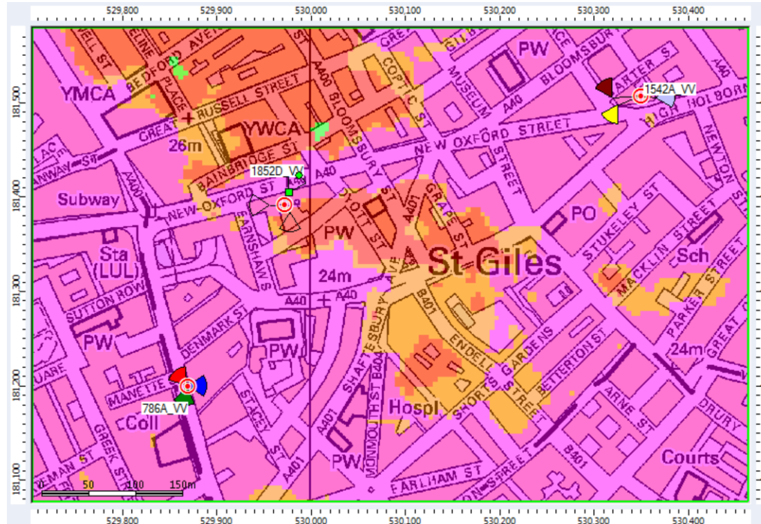
Fig. 2: Existing voice coverage (1852 decommissioned)
