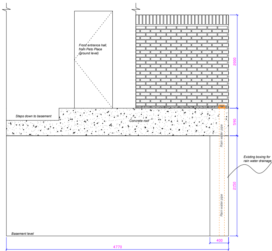
SECTION - A
