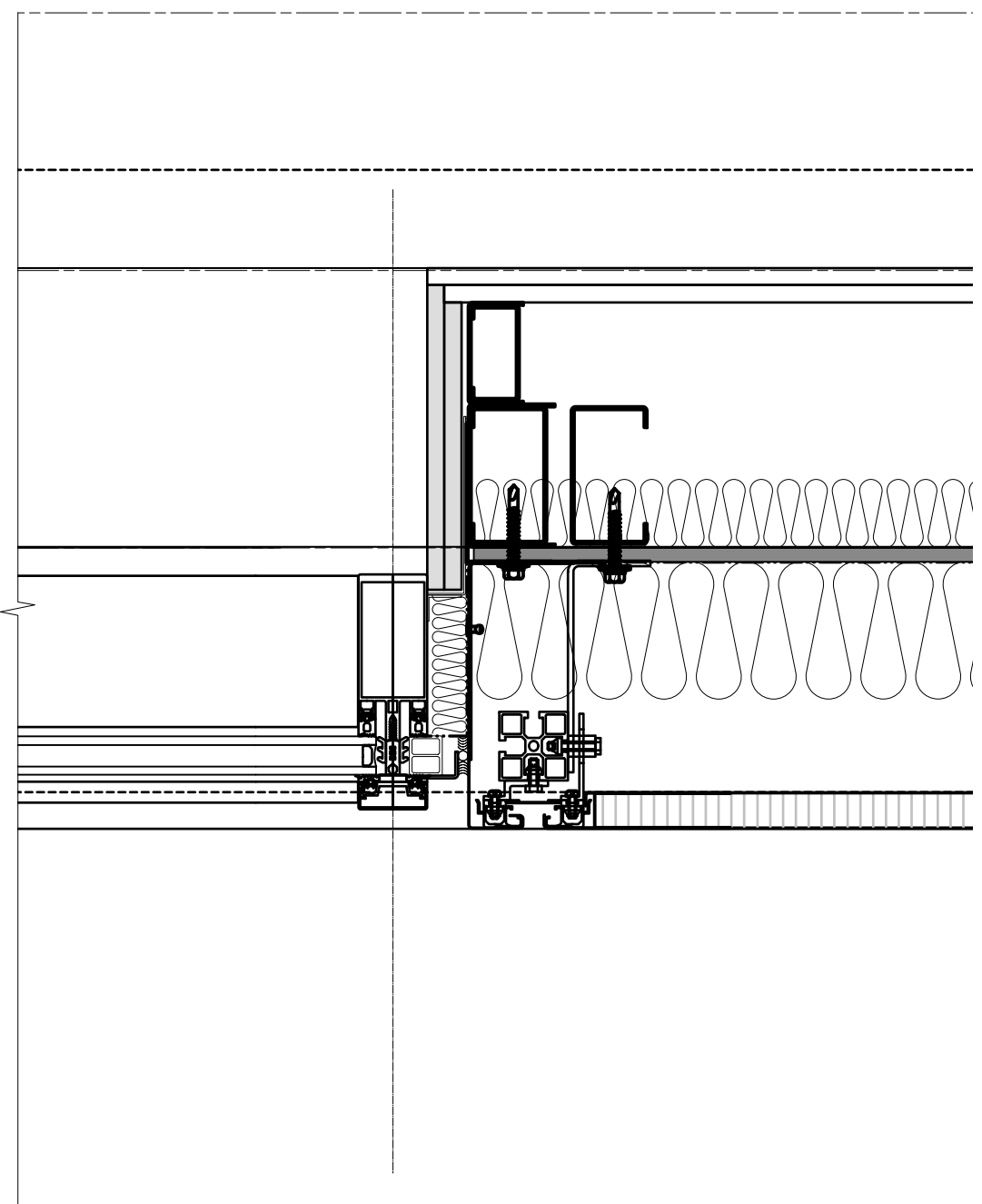
6 Horizontal Section 1:5
