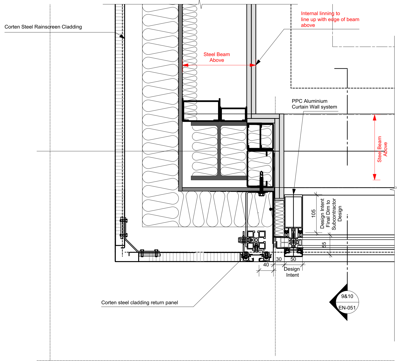
3 Horizontal Section 1:5
