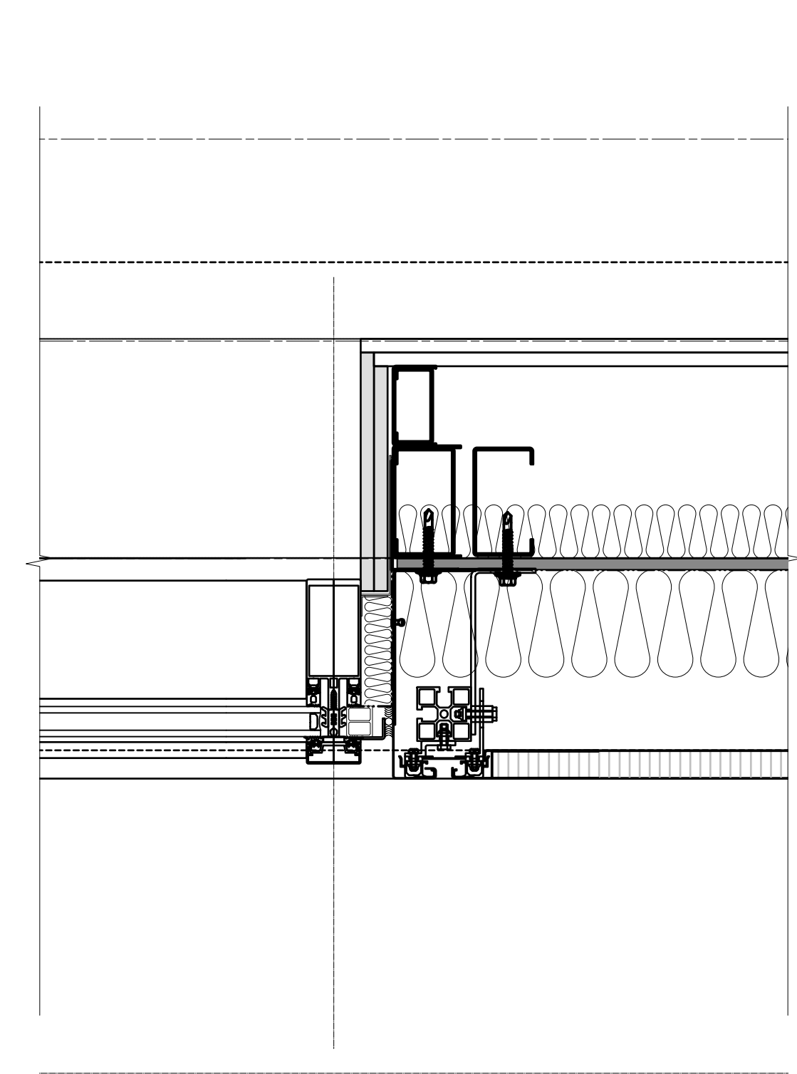
4 Horizontal Section 1:5
