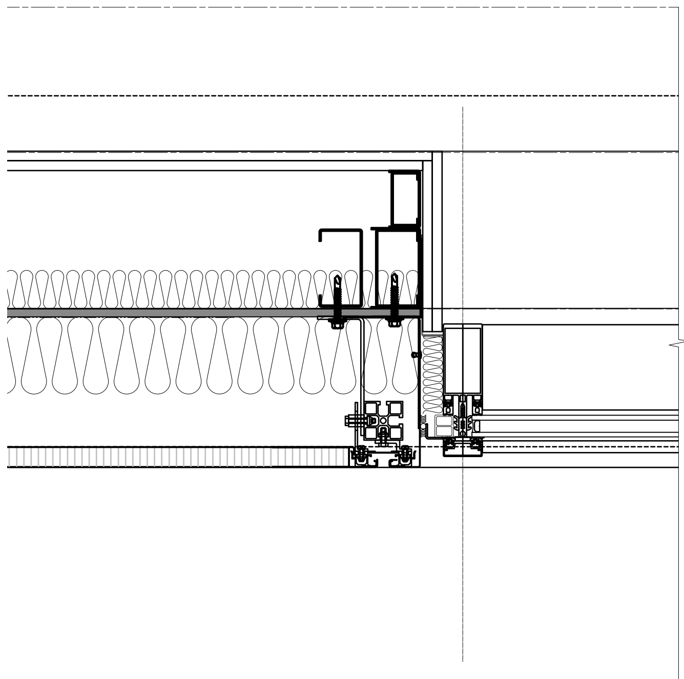
5 Horizontal Section 1:5
