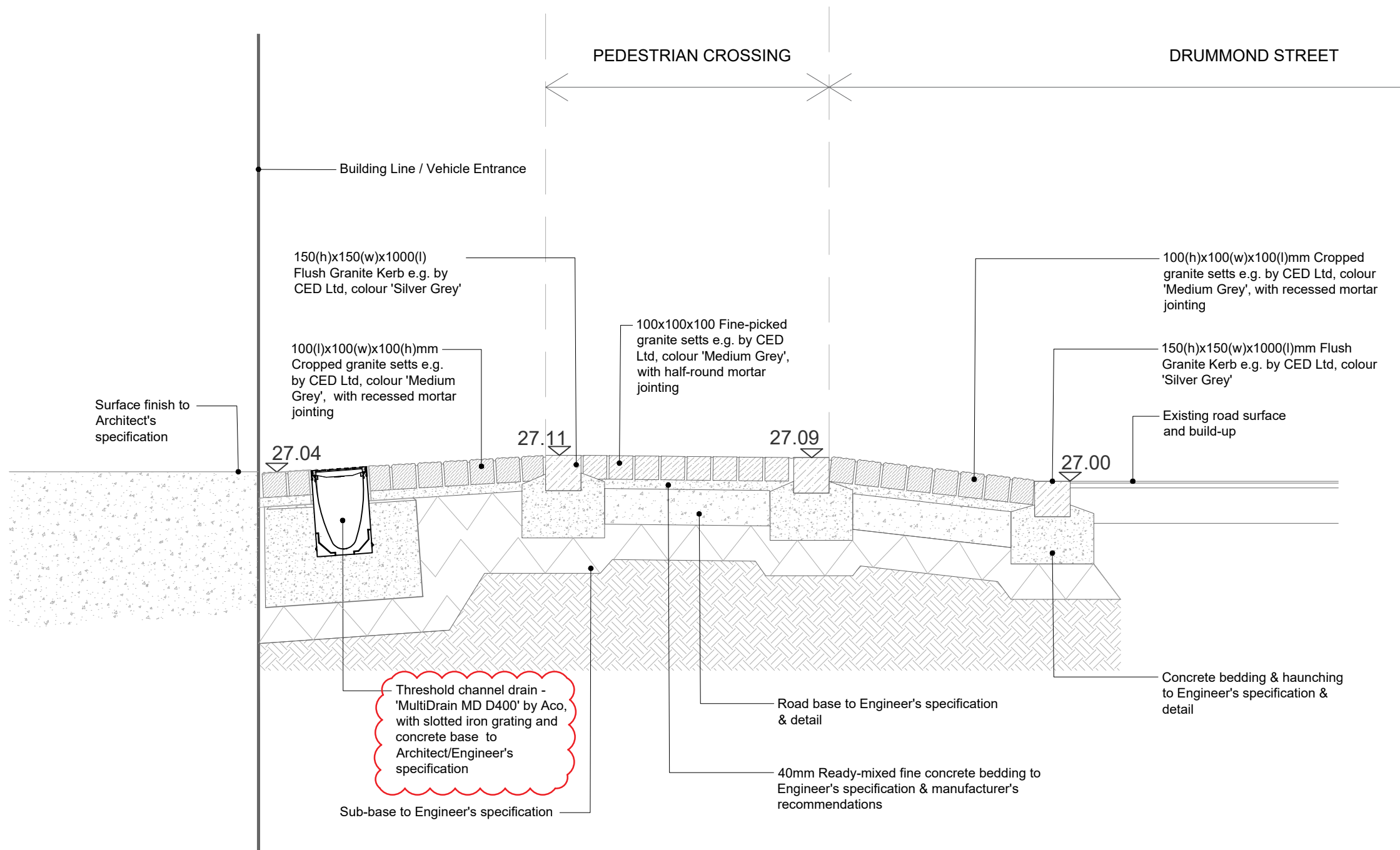
01 Granite Sett Paving At Drummond Street Vehicular Entrance 301 Scale 1:20
