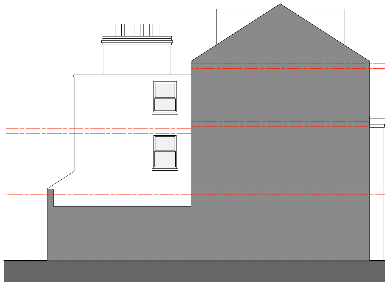
Proposed Side Elevation / Section East 1:100
