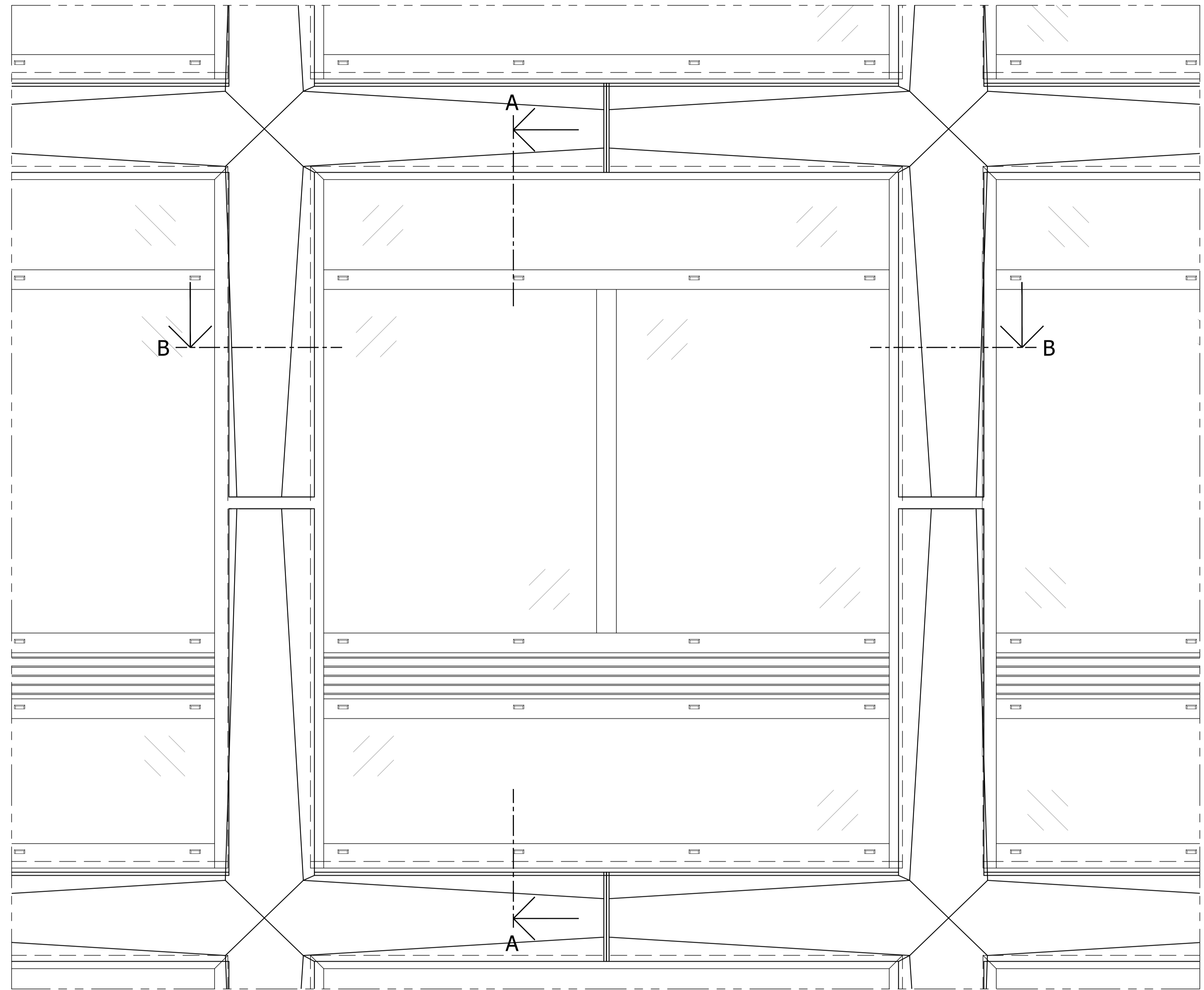
TOWER WINDOWS - EXTERNAL ELEVATION
