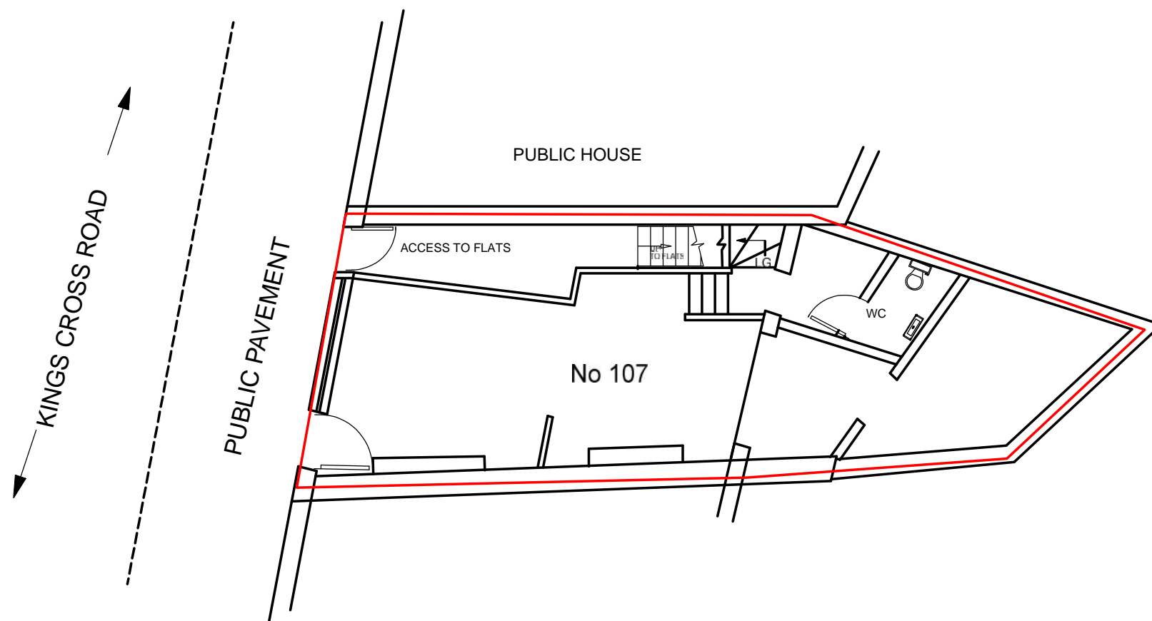
GROUND FLOOR LOCATION PLAN
