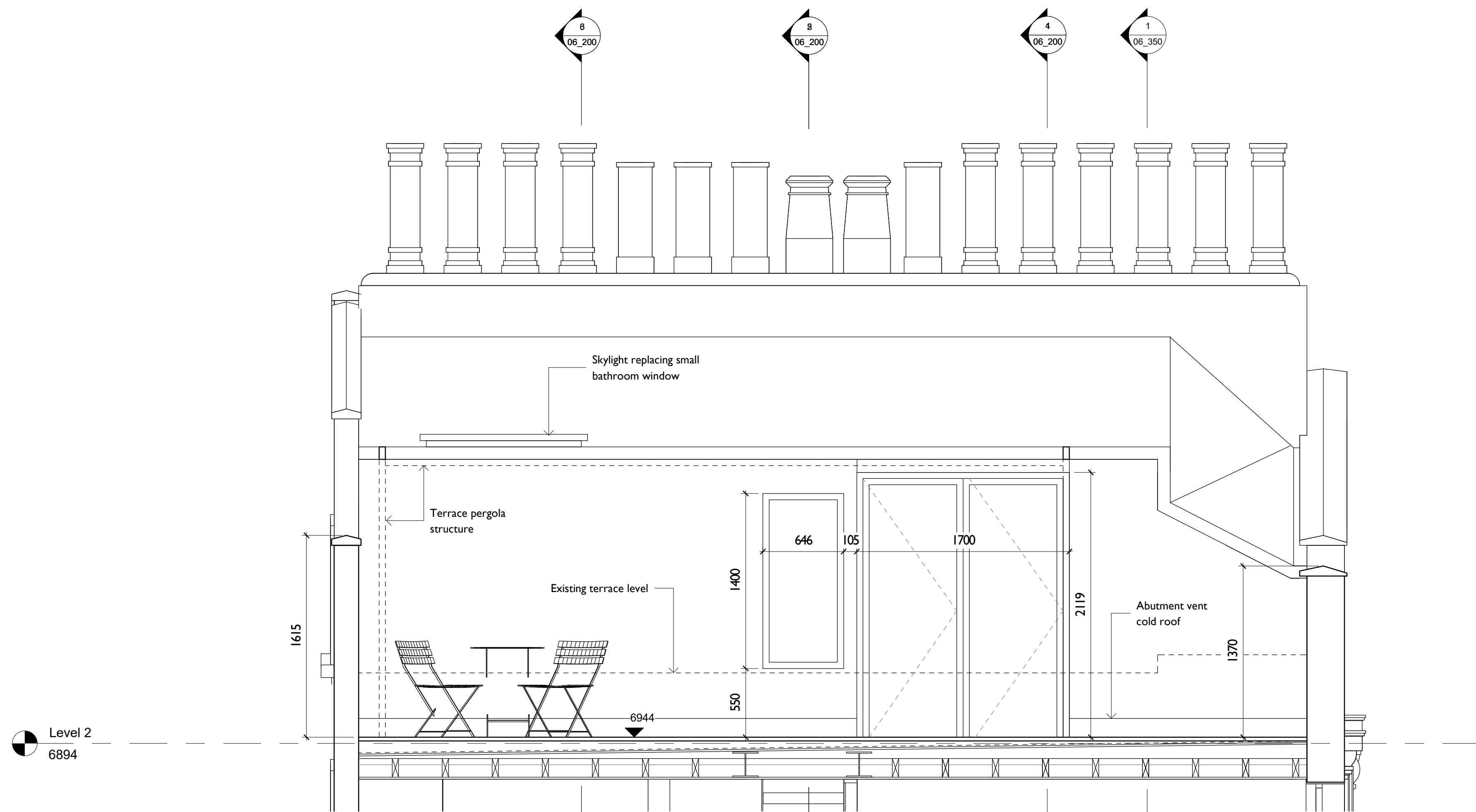
1 PROPOSED 1 : 25
