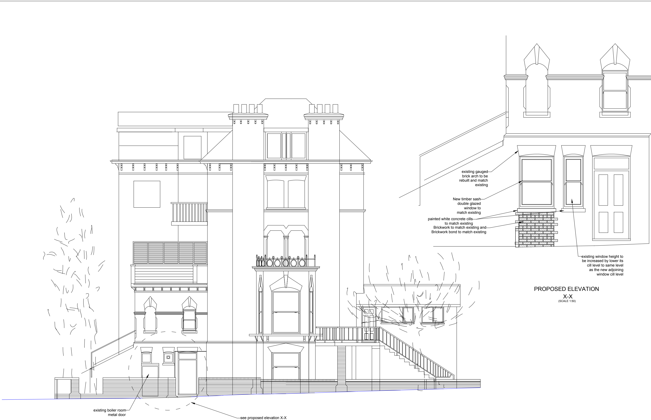
EXISTING NORTH ELEVATION ELEVATION (VIEW FROM PRINCE ARTHUR ROAD)
