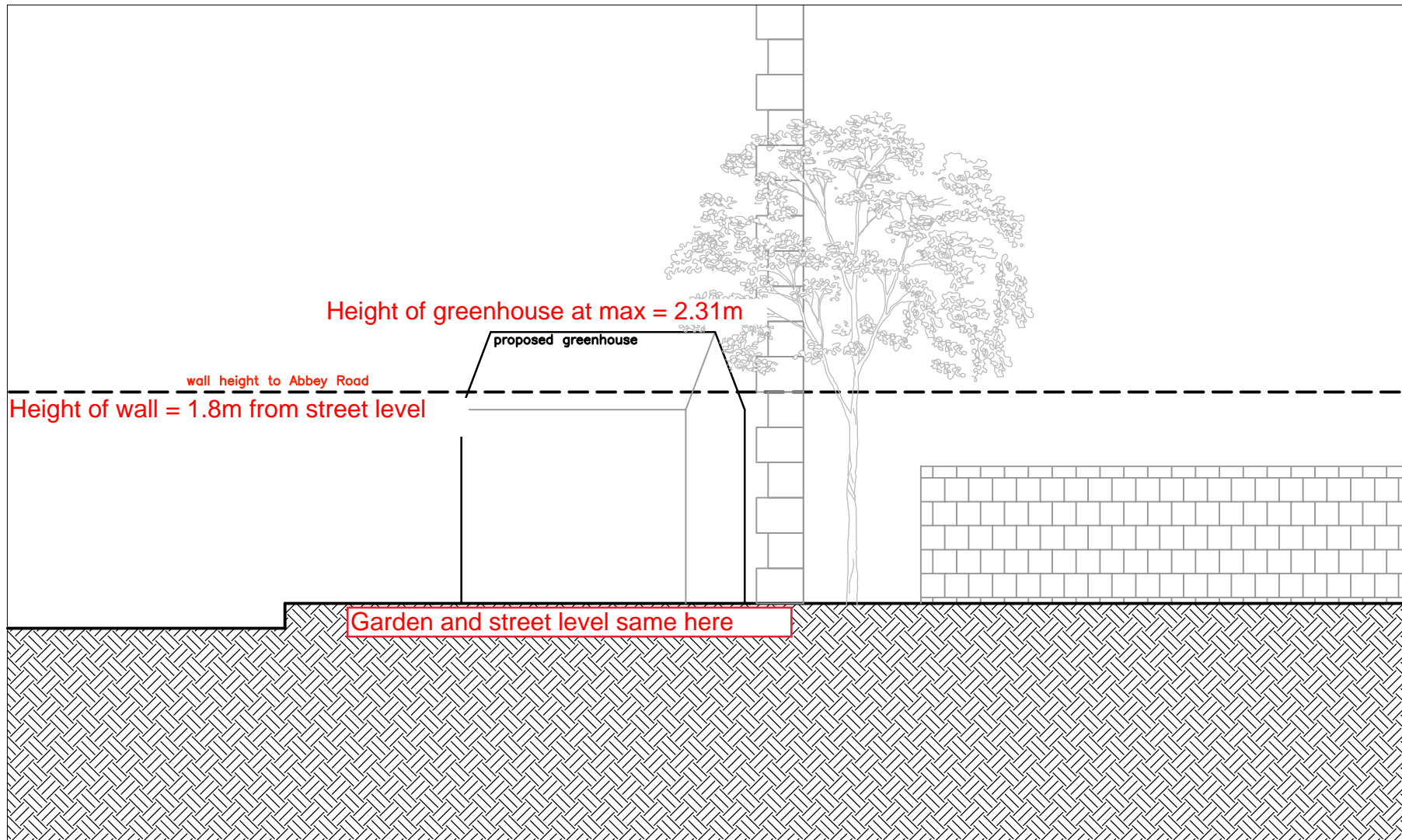
Elevation of proposed greenhouse looking south 1:50 when printed at A4
