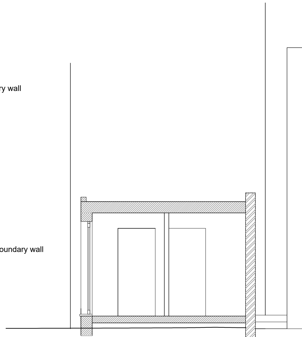
Section "B"
