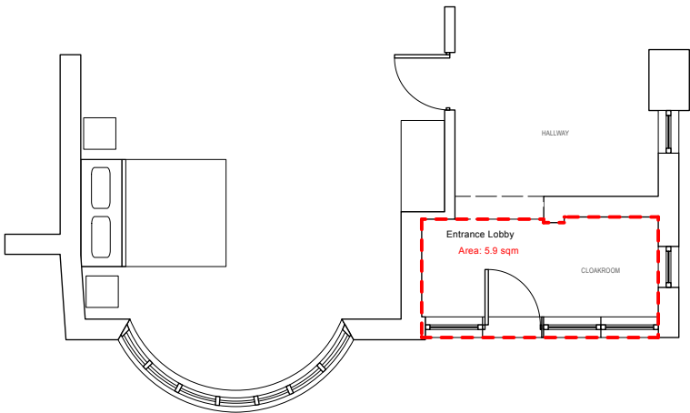
PLAN OF GROUND FLOOR ENTRANCE
