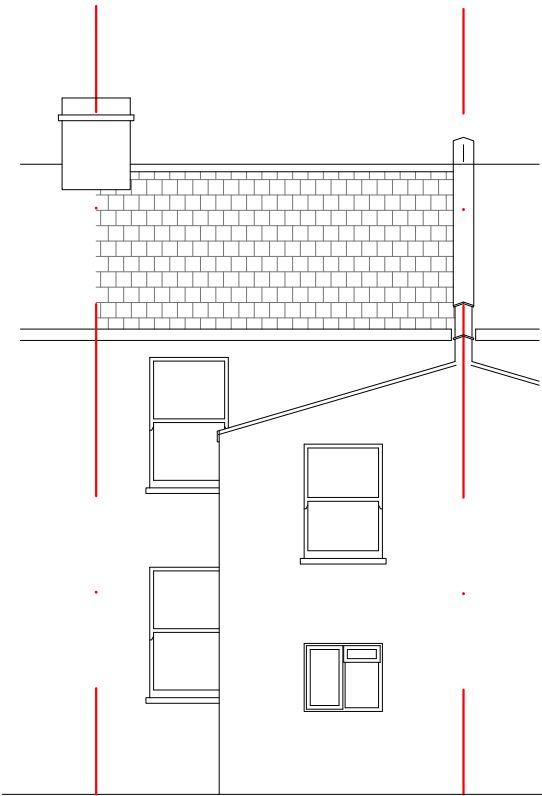
REAR ELEVATION
