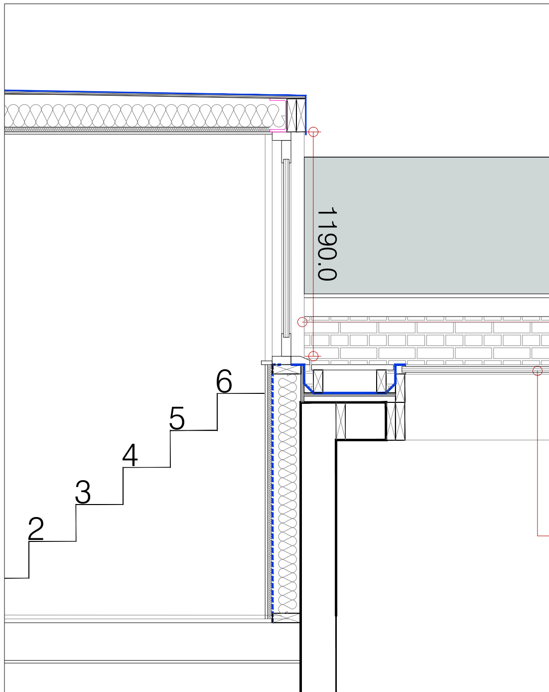
SECTION THROUGH WINDOW /DOOR
