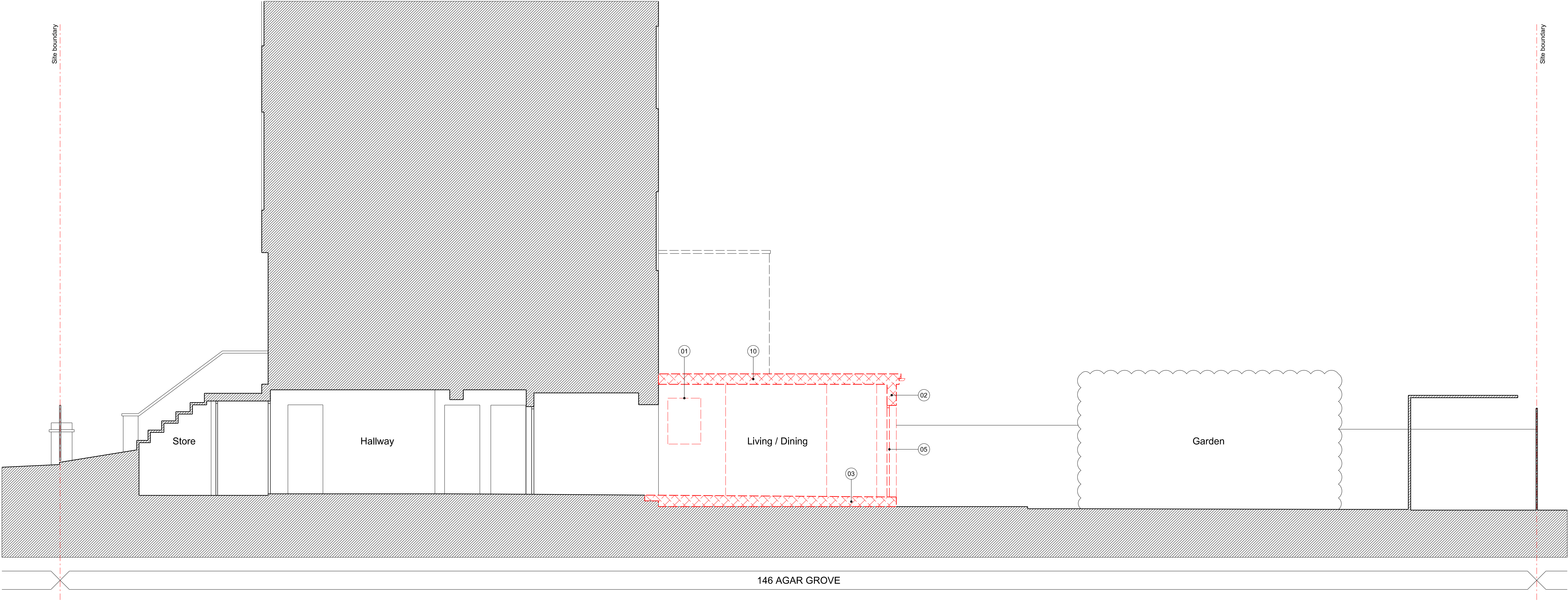
Existing Section AA
