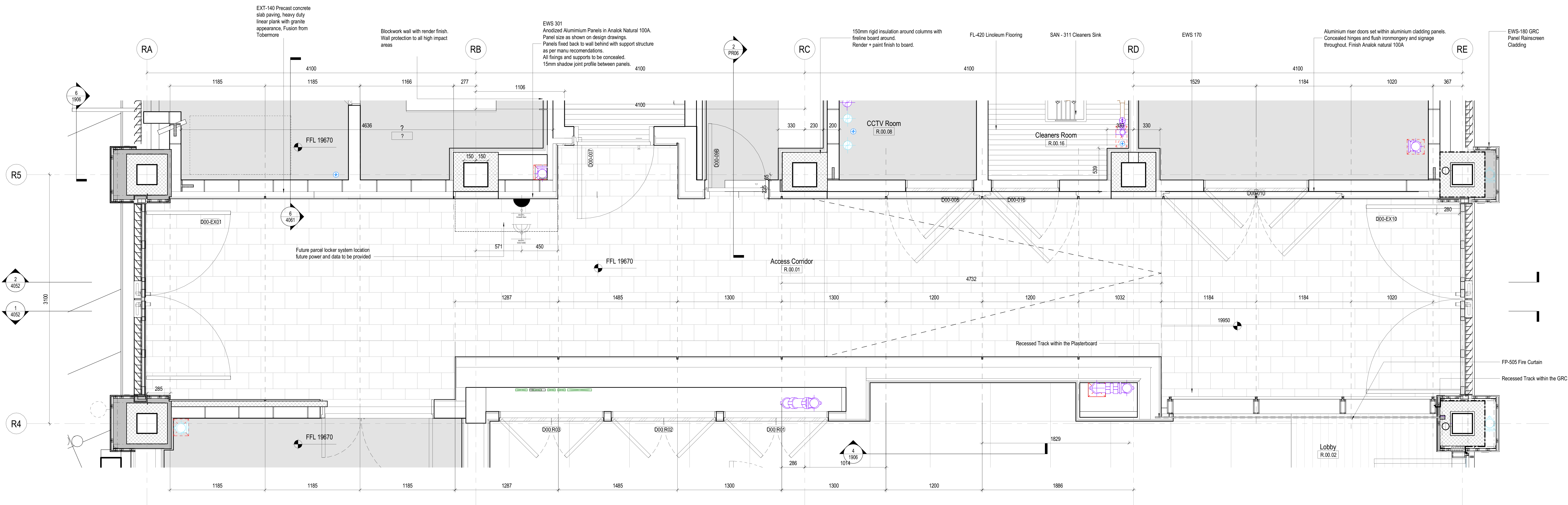
1 Access Corridor Enlarged Plan 1 : 20
