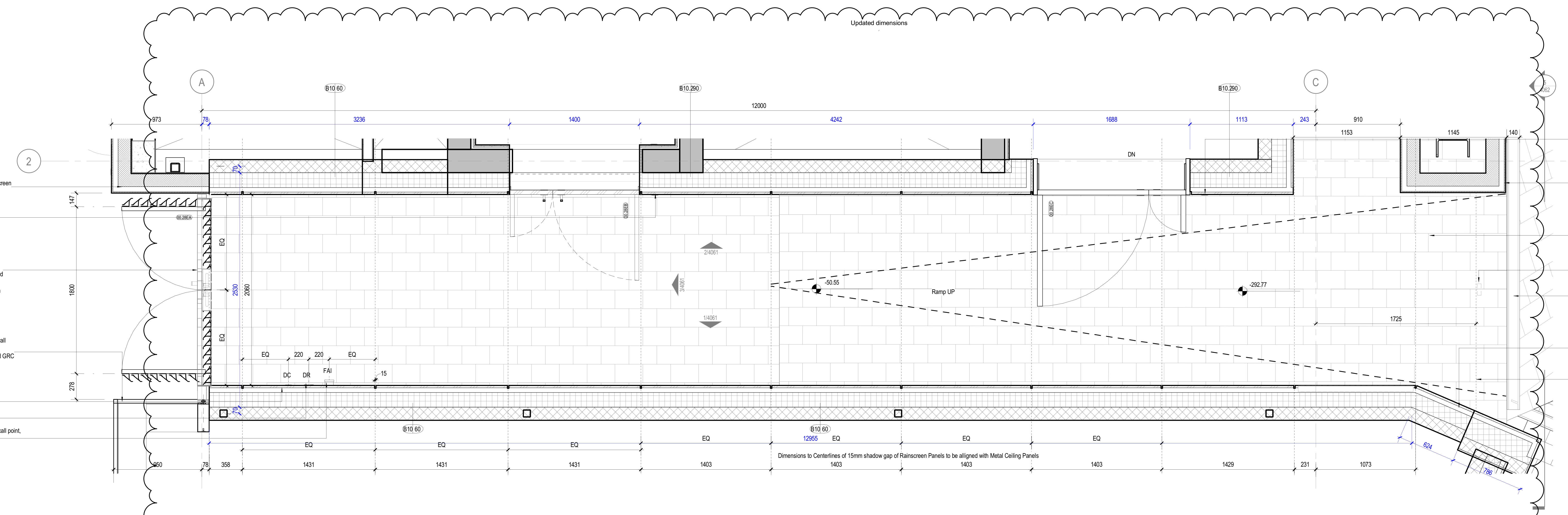
1 West Access Corridor L00 - Enlarged Plan 1:20 Referencing View: 1/ A1100
