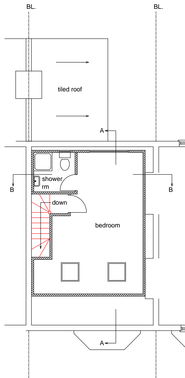
Third Floor Plan 'As proposed' Scale: 1/100
