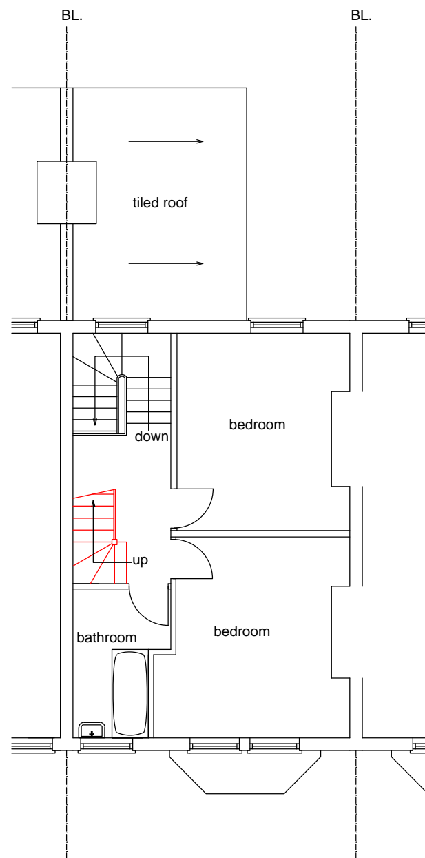
Second Floor Plan 'As proposed' Scale: 1/100
