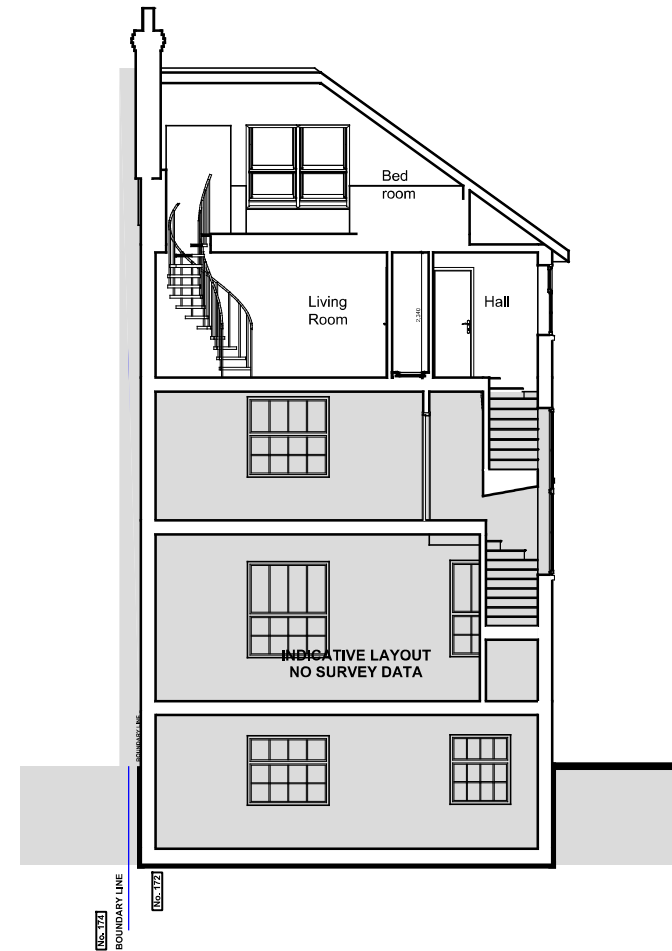
Section BB
