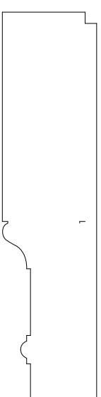
3. Existing mouldings profile 1:2
