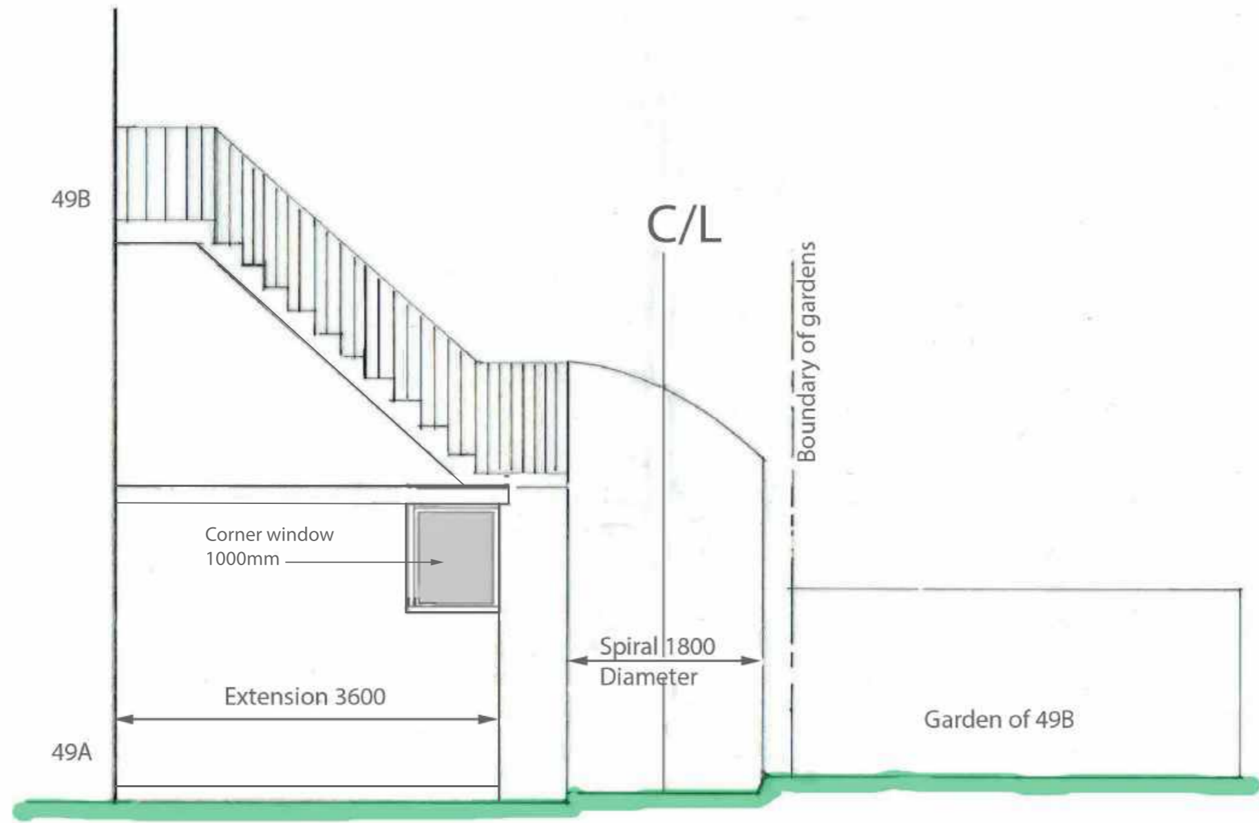
East Elevation Proposed
