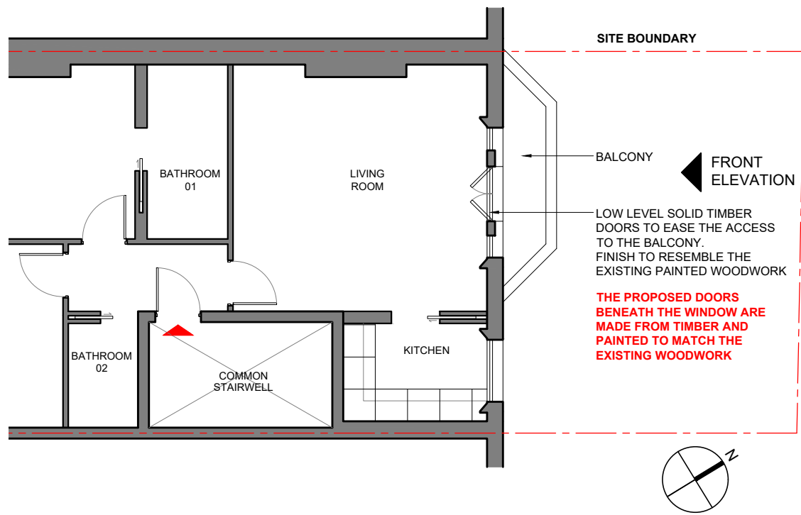
1 PROPOSED FIRST FLOOR PLAN_ SCALE 1:100 @ A3
